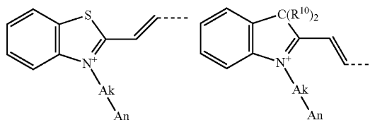
(IIIa-1)
