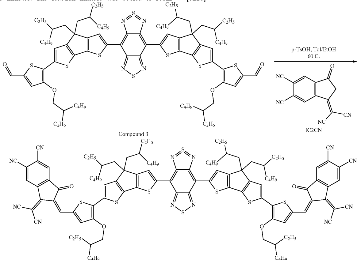
Compound Example 1
