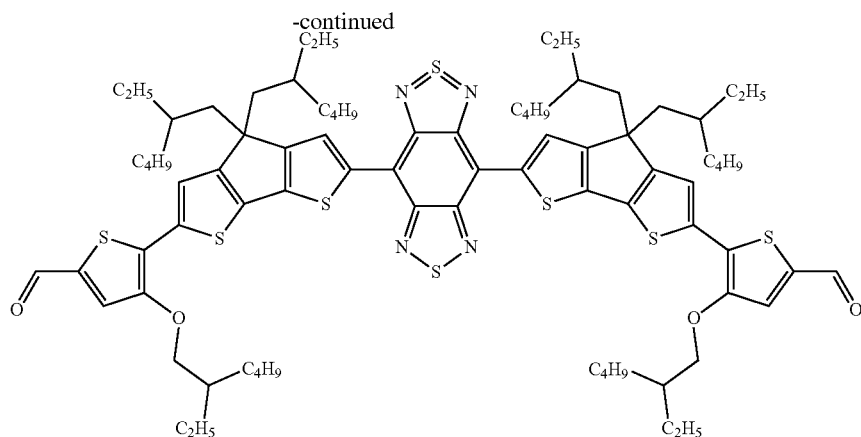
Compound 3
