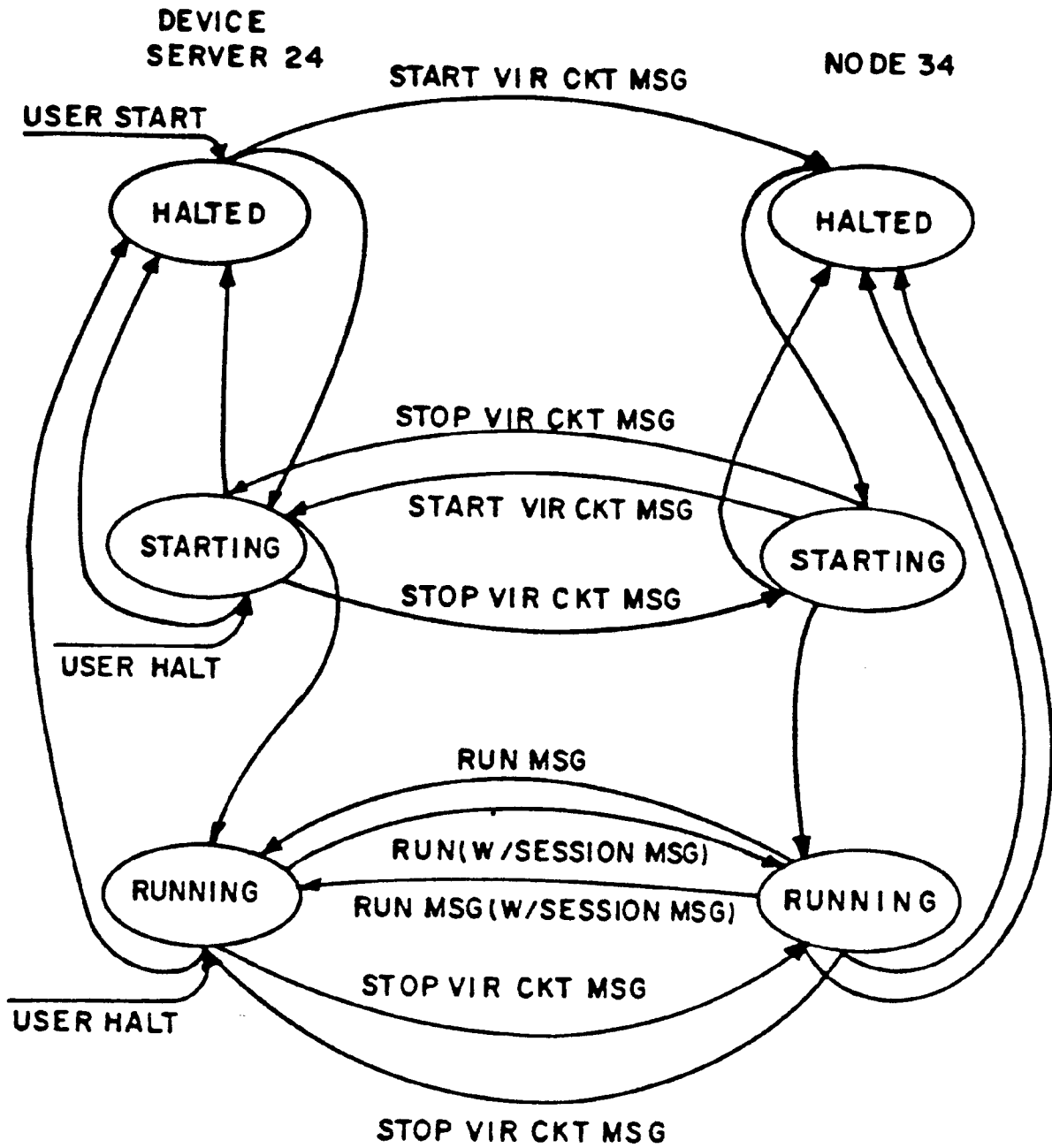
VIRTUAL CIRCUIT STATE DIAGRAM
