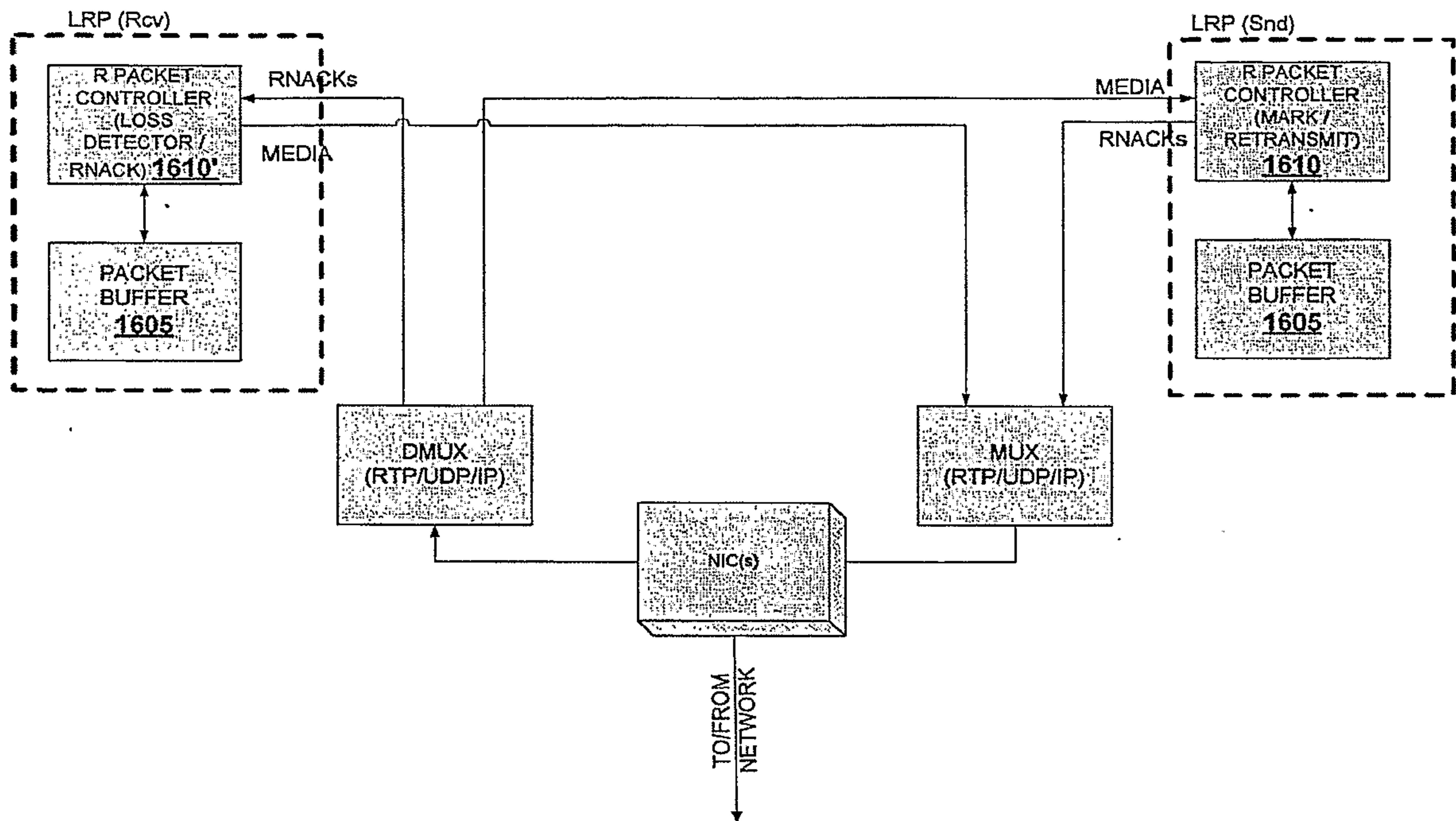
FIG. 18: SERVER WITH LRP USING RTP
