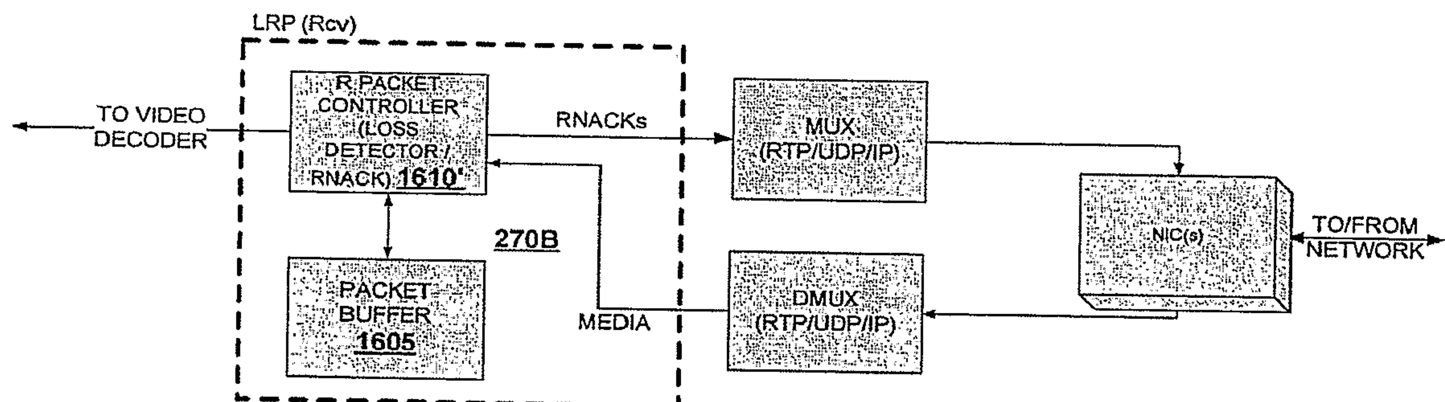
FIG. 17: RECEIVING TERMINAL WITH LRP USING RTP
