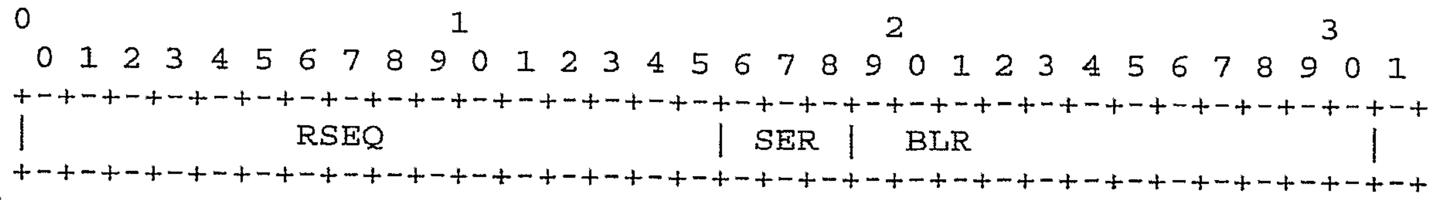
FIG. 20: RNACK FEEDBACK CONTROL INFORMATION (FCI) FIELD
