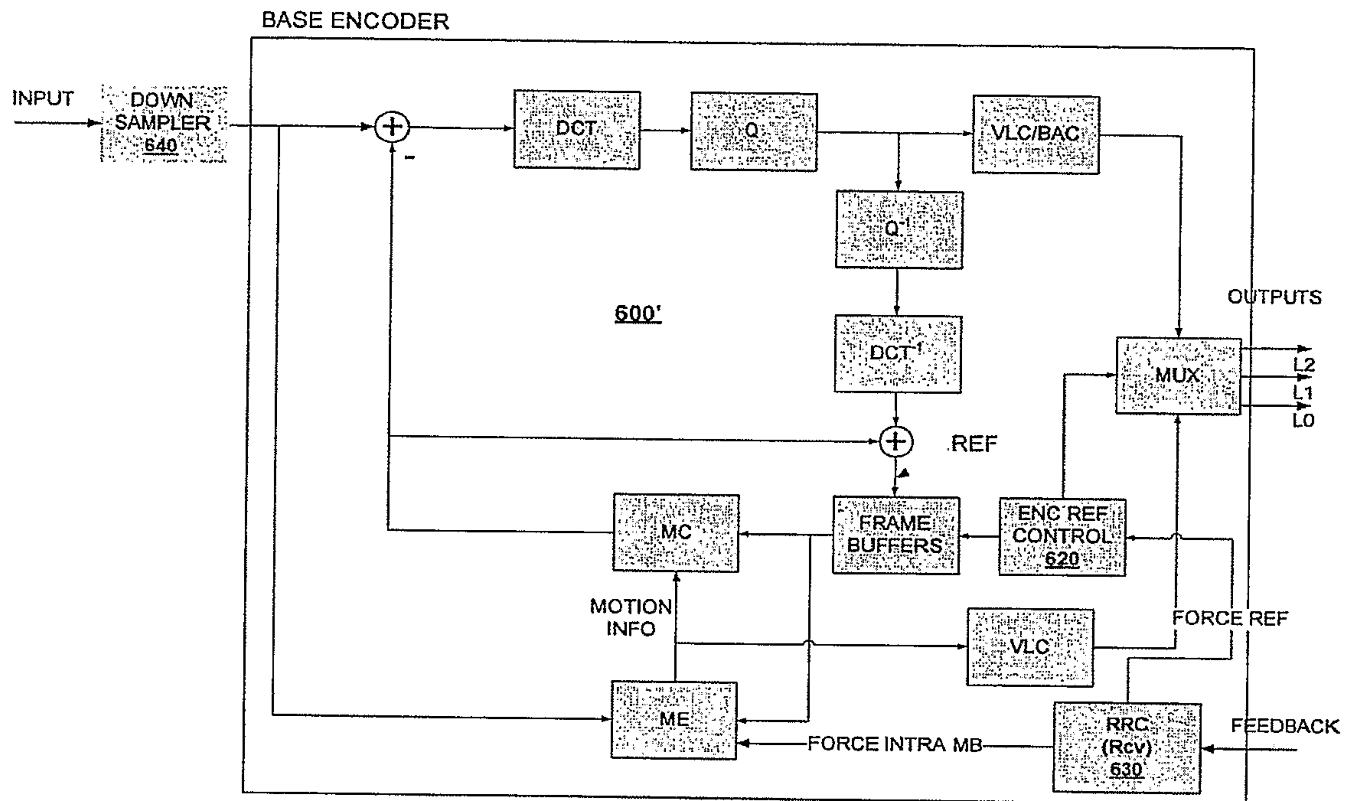
FIG. 7: VIDEO ENCODER (BASE AND TEMPORAL ENHANCEMENT LAYERS)
