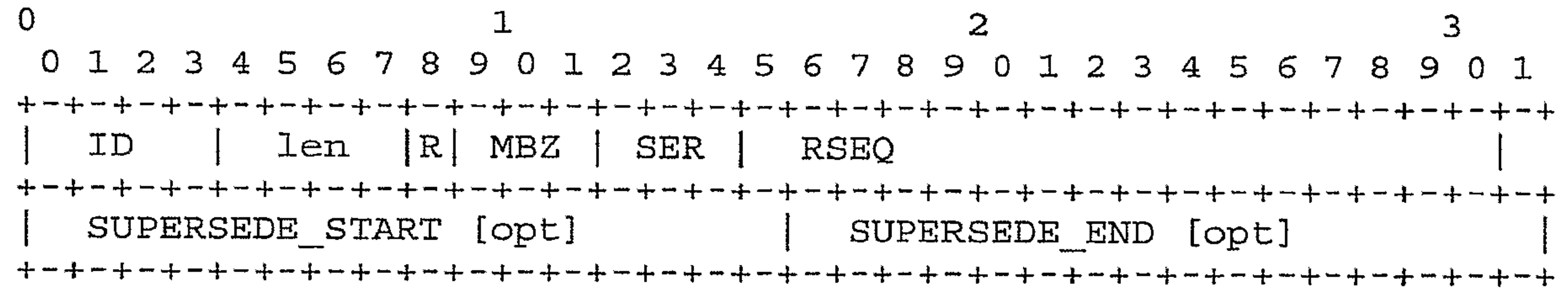
FIG. 19: RTP HEADER EXTENSION FOR RTP PACKETS
