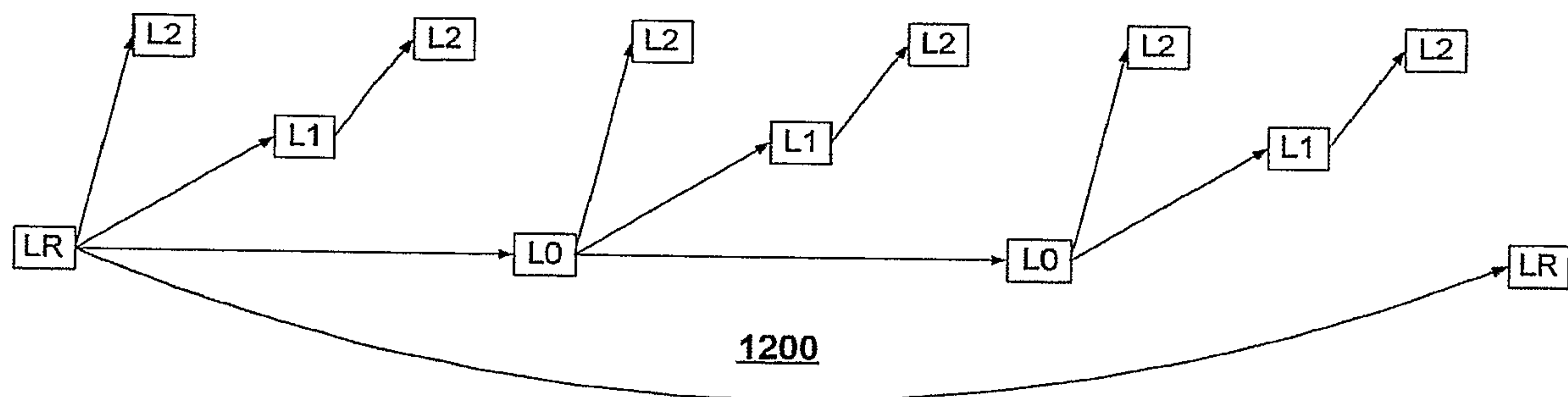
FIG. 12: PICTURE CODING STRUCTURE WITH LR PICTURES
