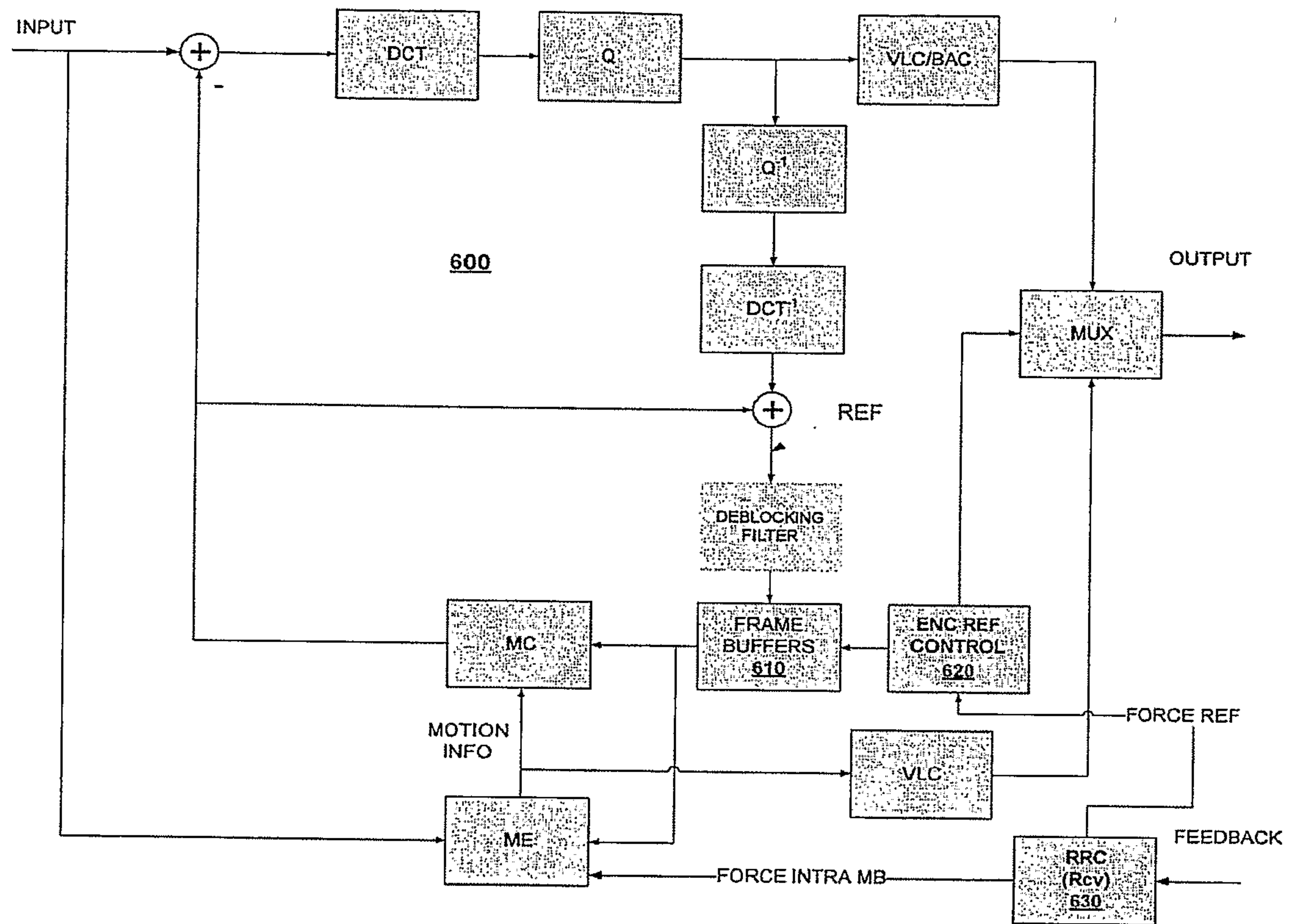
FIG. 6: VIDEO ENCODER
