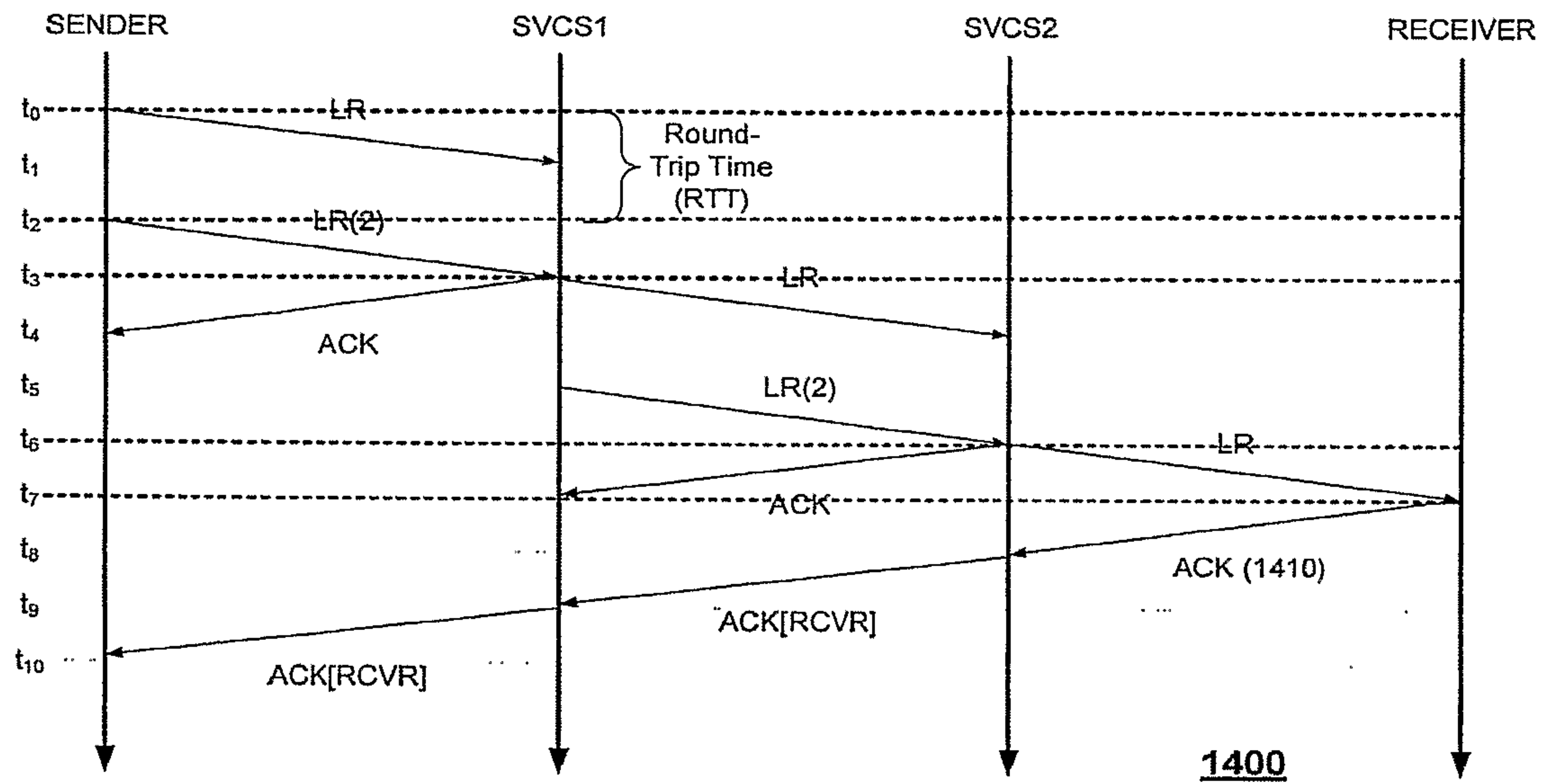
FIG. 14: THE LR PROTECTION (LRP) PROTOCOL USING POSITIVE ACKNOWLEDGMENTS
