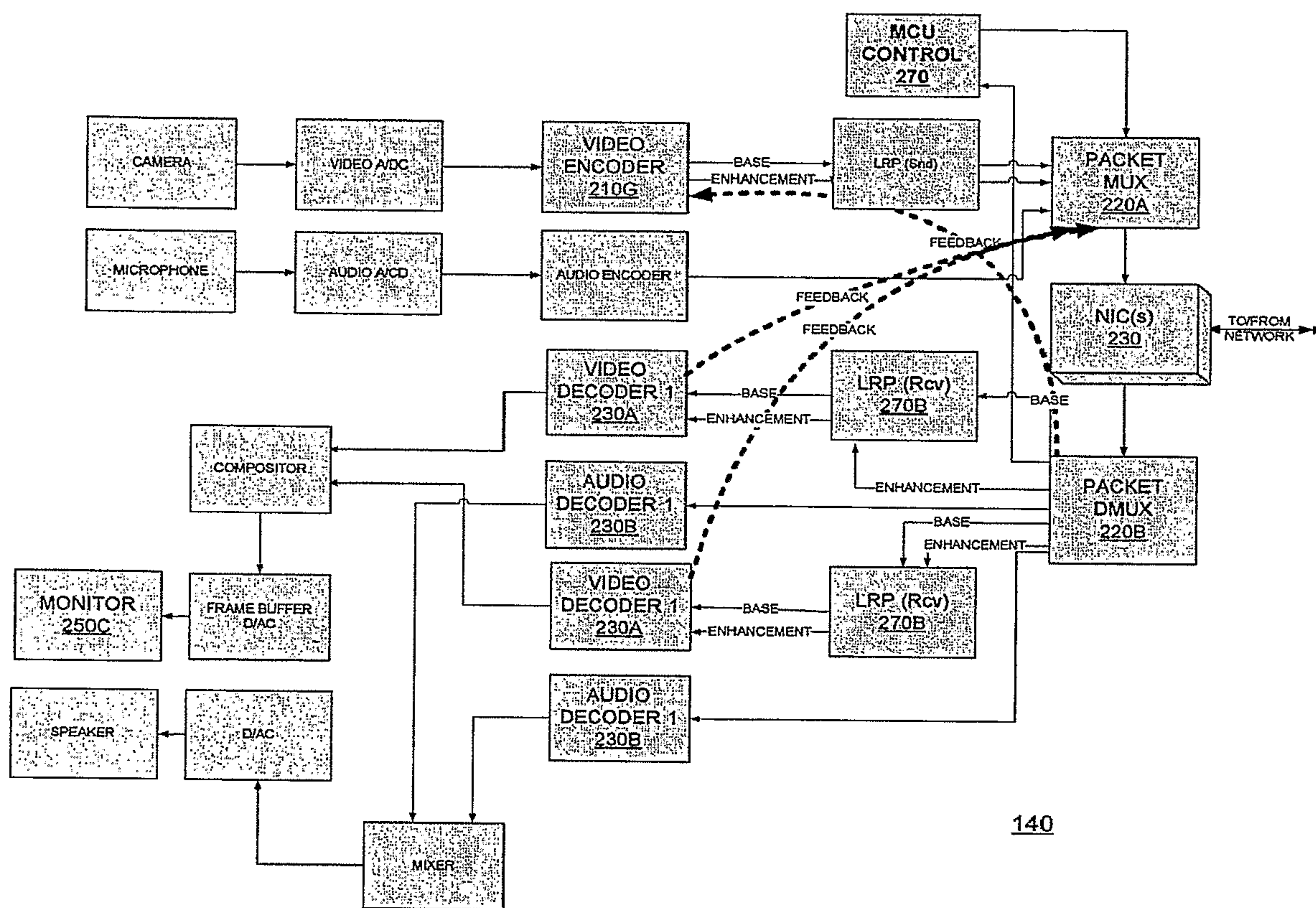
FIG. 3: END-USER TERMINAL (SCALABLE OR SIMULCAST CODING)
