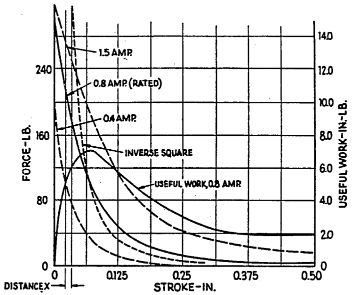
FLAT-FACED PLUNGER MAGNET AND ITS FORCE-STROKE CURVES
