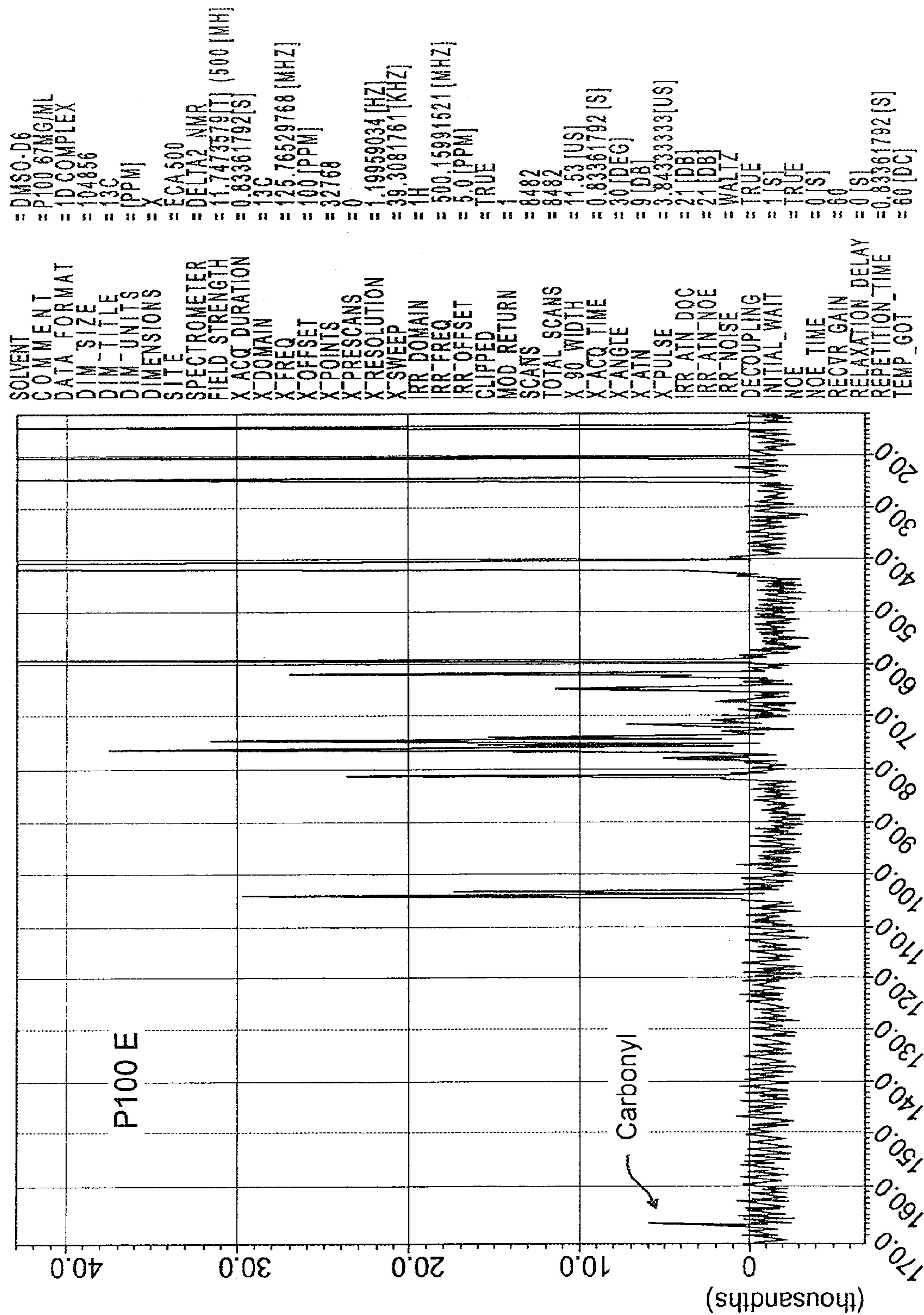
FIG. 40 K X : parts per Million : 13C
