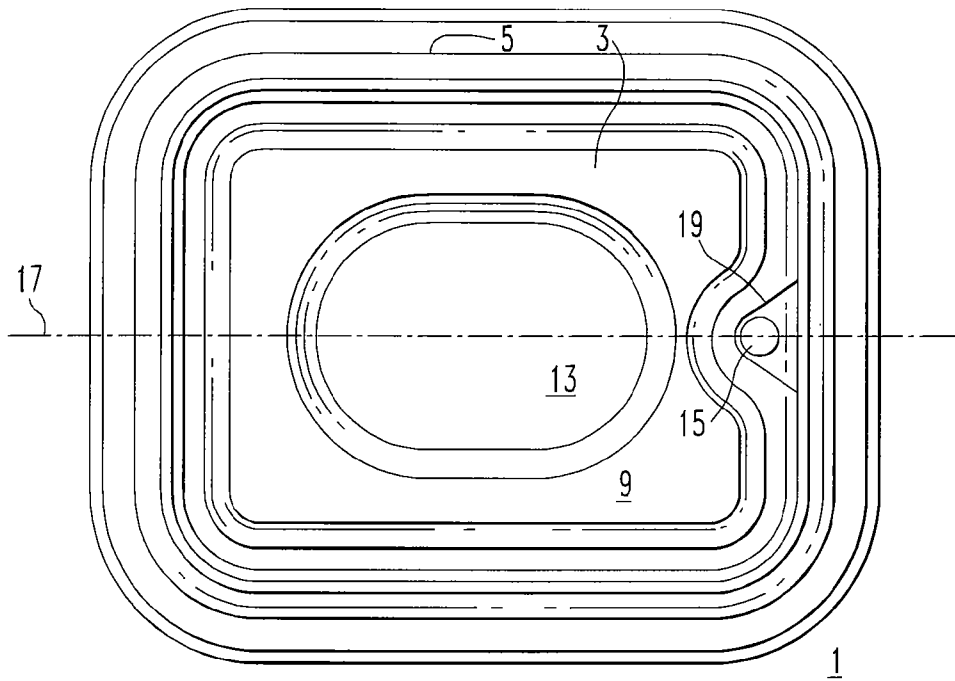
FIG. 1 PRIOR ART
