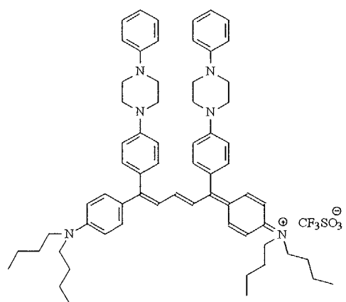
DYE 4 (824 nm, 1.74 \times 10^{-5} )
