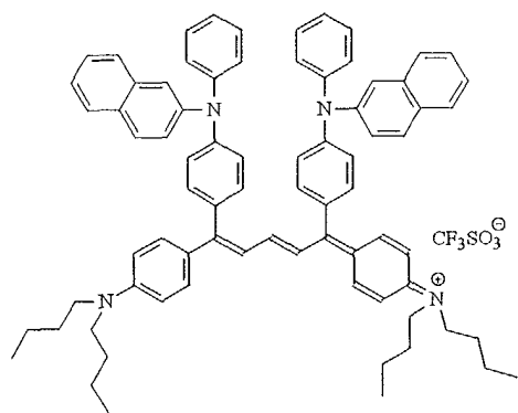
DYE 7 (842 nm, 8.9 \times 10^{-4} )
