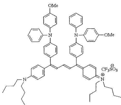
DYE 8 (839 nm, 1.18 \times 10^{-5} )
