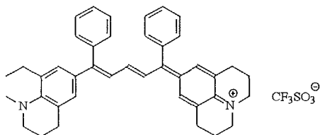
DYE 1 (880 nm, 1.26 \times 10^{-5} )
