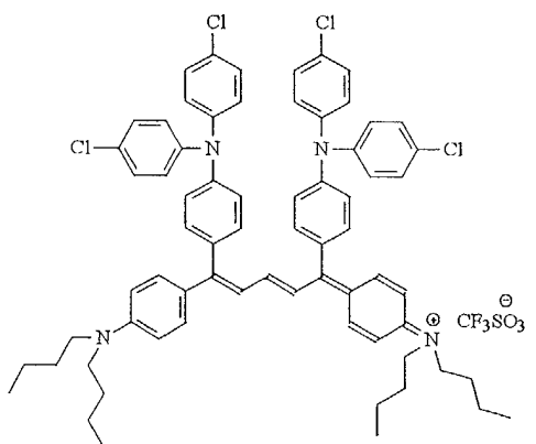
DYE 5 (843 nm, 1.65 \times 10^{-5} )
