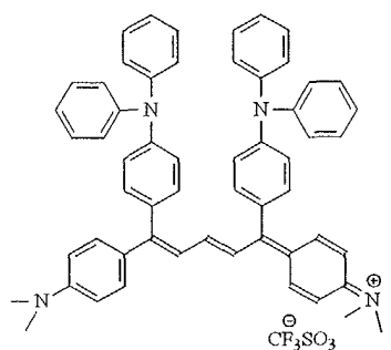
DYE 10 (838 nm, 1.0 \times 10^{-5} )
