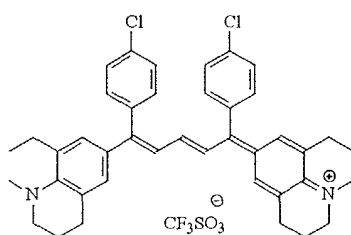
DYE 12 (890 nm, 1.24 \times 10^{-5} )
