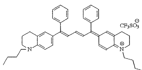
DYE 11 (860 nm, 9.6 \times 10^{-4} )
