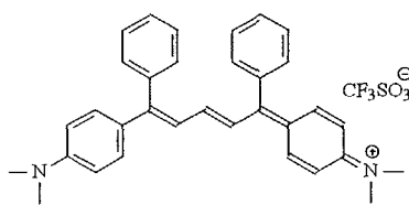
DYE 2 (830 nm, 1.2 \times 10^{-5} )
