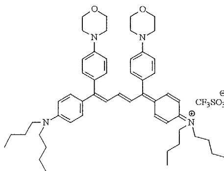
DYE 3 (823 nm, 1.55 \times 10^{-5} )
