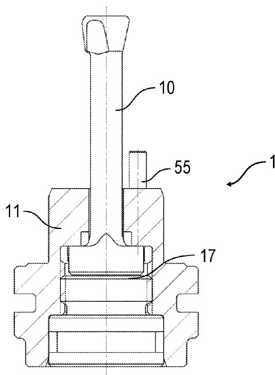
Fig. 13A Section F-F
