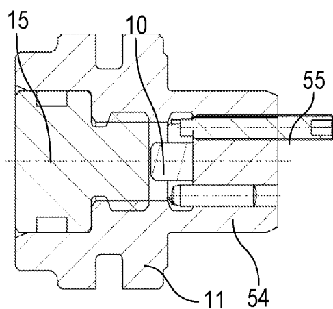
Fig. 13A Section F-F
