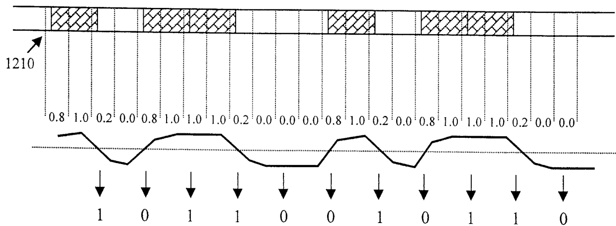
FIG. 12 Extracting the tag from the MPEG bitstream
