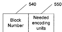
Receiver feedback format
