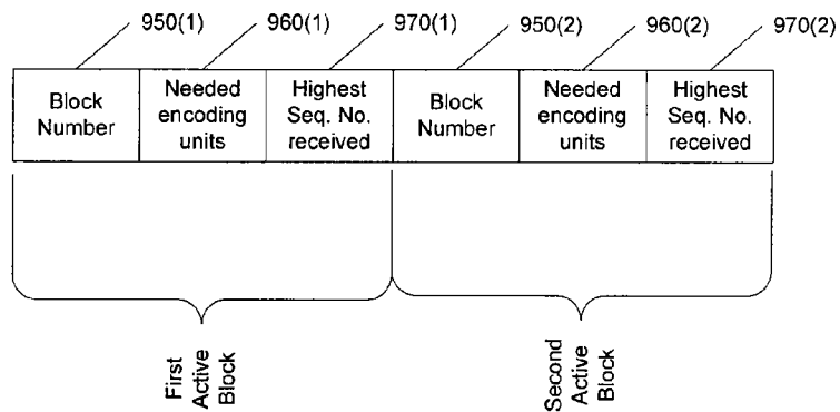
Receiver feedback format
