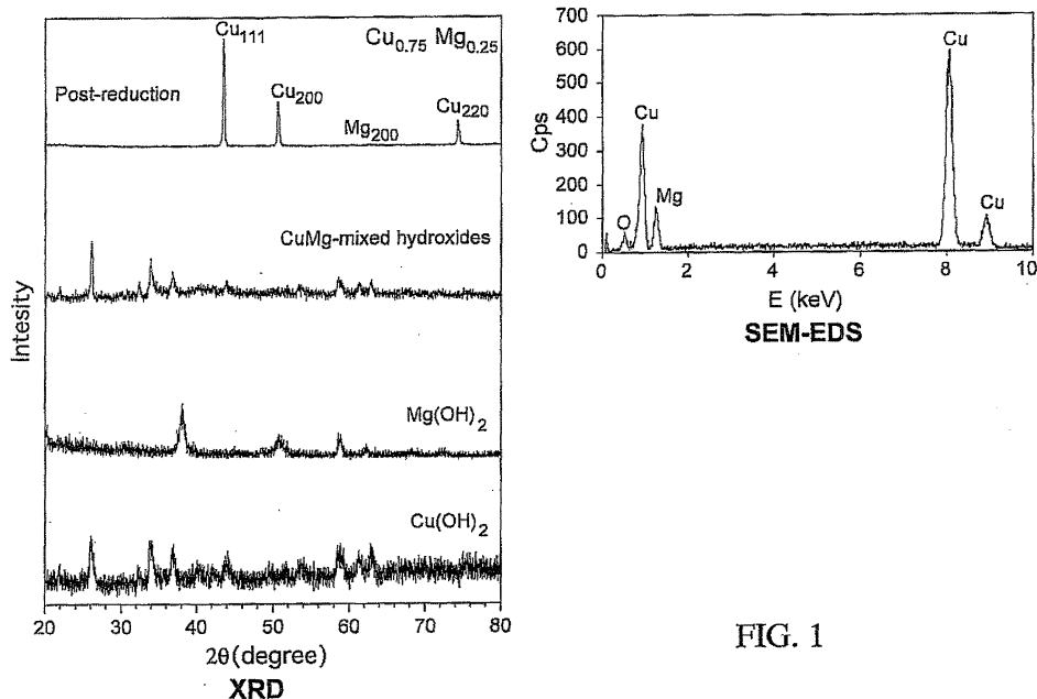
Characterization of Cu_{0.75}Mg_{0.25} Nanoalloy 1
