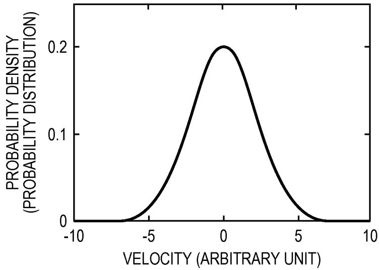
M-B "VELOCITY (ONE-DIMENSIONAL PROJECTION)" DISTRIBUTION
