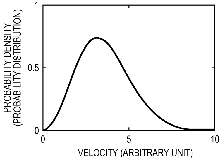
M-B "VELOCITY" DISTRIBUTION
