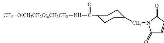
mPEG-MCH-MAL
