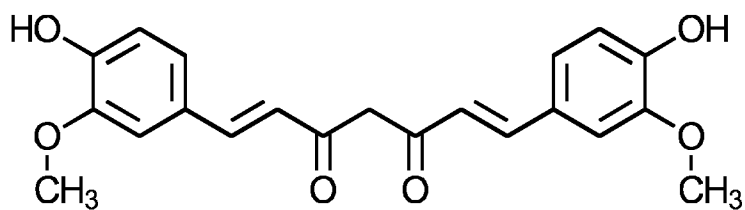
Keto form of curcumin
