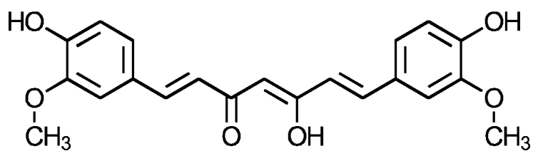
Enol form of curcumin
