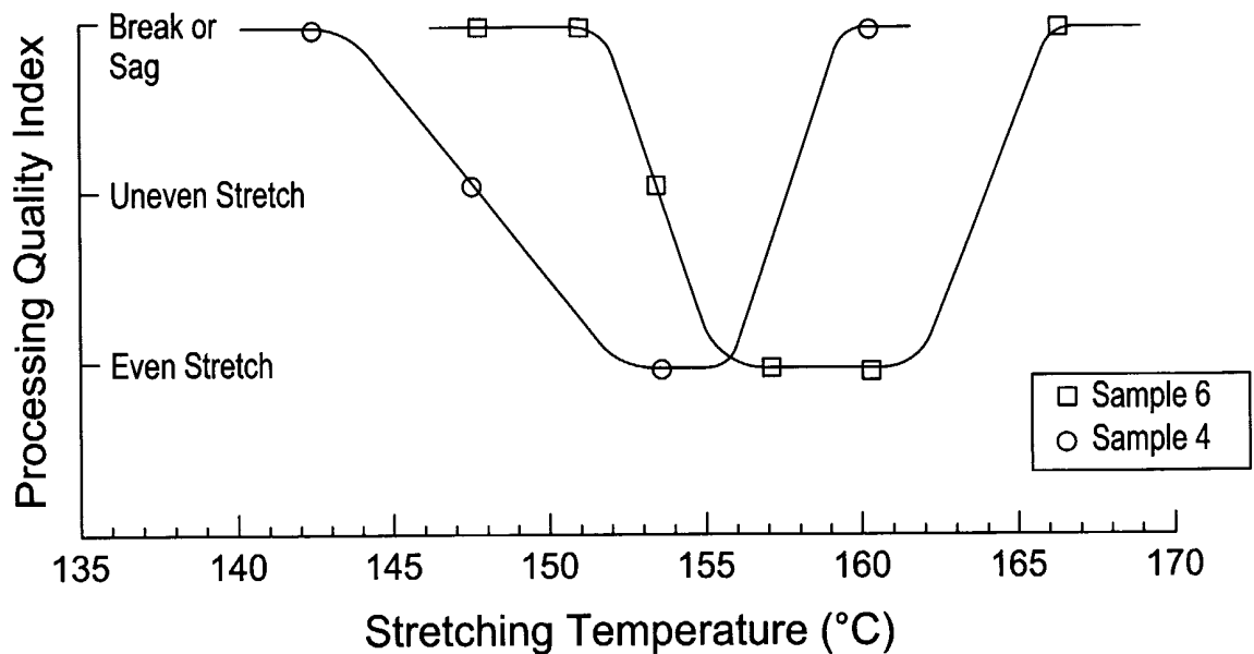
Fig. 4A Processing Window During Biaxial Stretching
