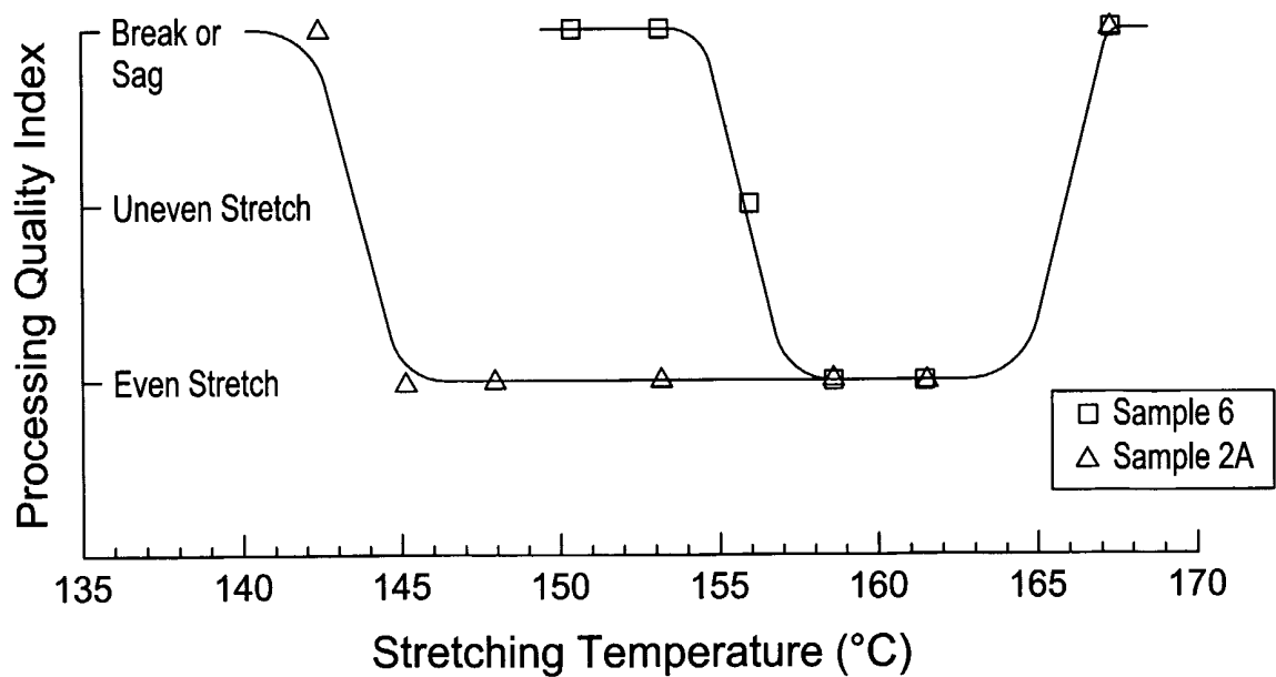
Fig. 4B Processing Window During Biaxial Stretching
