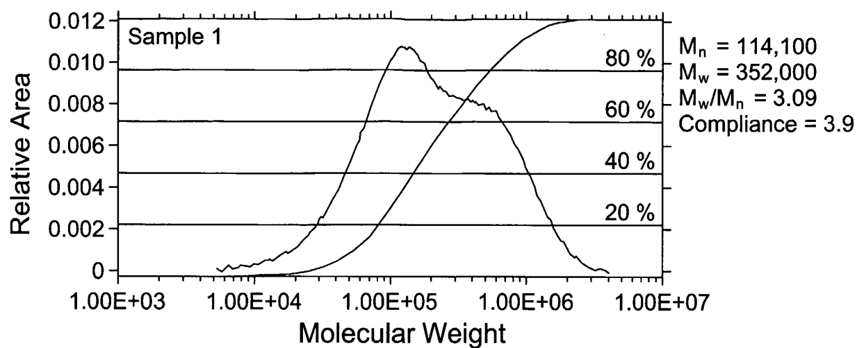
Fig. 1A GPC Molecular Weight Distributions
