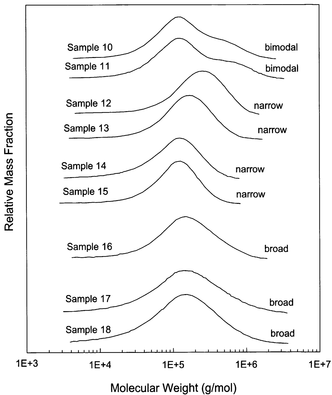
Fig. 6 GPC Molecular Weight Distribution
