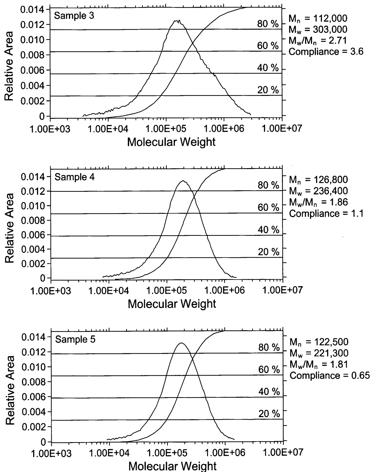
Fig. 1B GPC Molecular Weight Distributions
