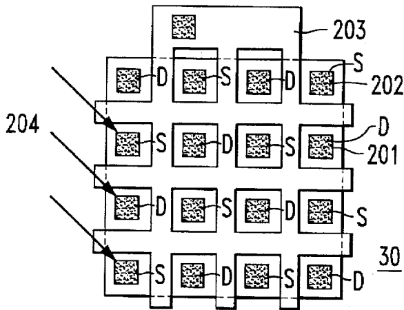
FIG. 2 PRIOR ART
