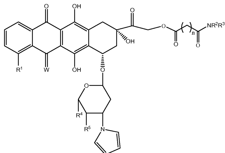
Formula (I)
