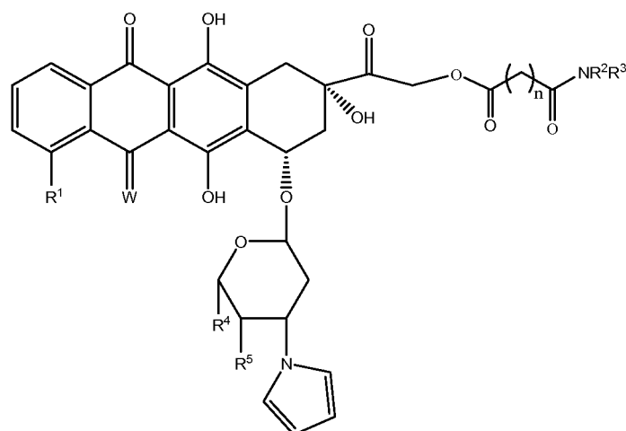
Formula (I)
