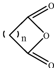
Formula (IV)
