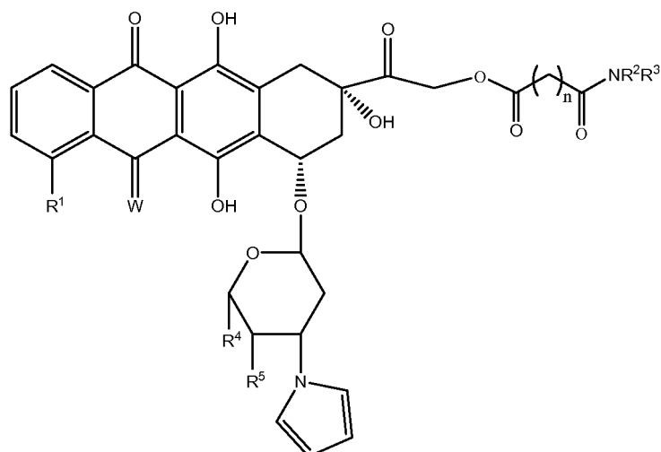
Formula (I)
