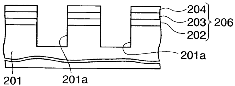
FIG. 1C (PRIOR ART)
