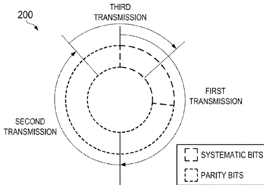
FIG. 2 (PRIOR ART)
