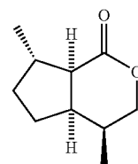
(9S,5S,1R,6R)-5,9-dimethyl-3-oxabicyclo[4.3.0]-nonan-2-one
