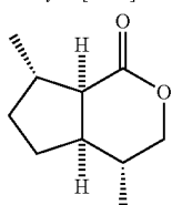
(9S,1R,5R,6R)-5,9-dimethyl-3-oxabicyclo[4.3.0]-nonan-2-one
