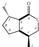
dihydronepetalactone of Formula 2 (9S, 5S, 1R, 6R)-5,9-dimethyl-3-oxabicyclo[4.3.0]nonan-2-one).
