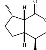
(1S,5S,9S,6S)-5,9-dimethyl-3-oxabicyclo[4.3.0]-nonan-2-one
