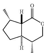
(1S,9S,5R,6R)-5,9-dimethyl-3-oxabicyclo[4.3.0]-nonan-2-one
