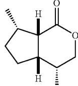
(1S,9S,6S,5R)-5,9-dimethyl-3-oxabicyclo[4.3.0]-nonan-2-one
