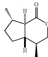
(9S,6S,1R,5S)-5,9-dimethyl-3-oxabicyclo[4.3.0]-nonan-2-one
