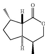
(1S,5S,9S,6R)-5,9-dimethyl-3-oxabicyclo[4.3.0]-nonan-2-one
