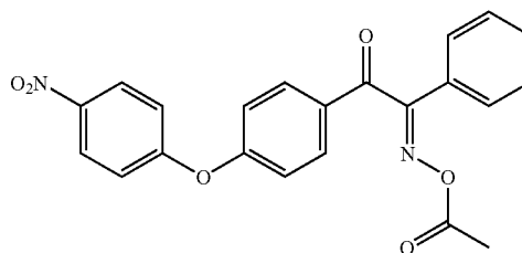
Compound No. 2
