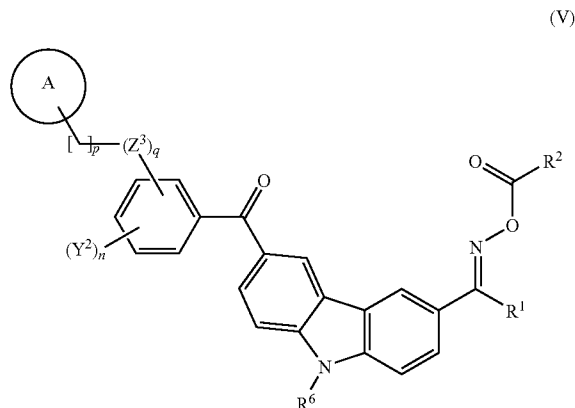
[Formula 39]
