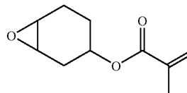
[Formula 31]
