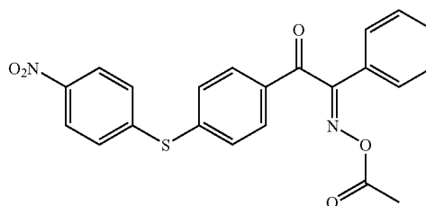
Compound No. 1
