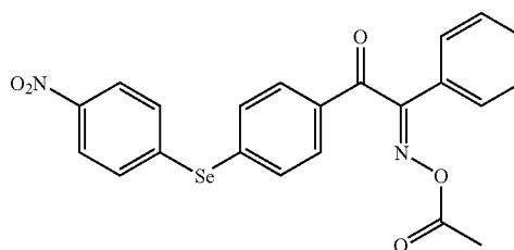
Compound No. 3
