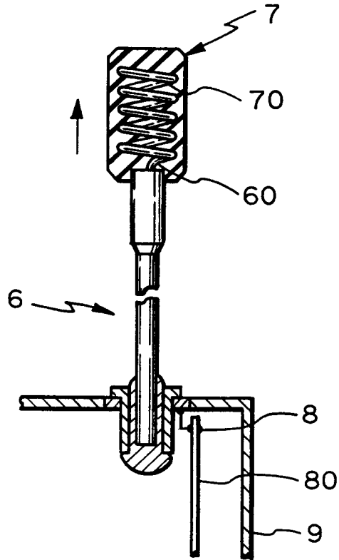
Fig. 6 PRIOR ART
