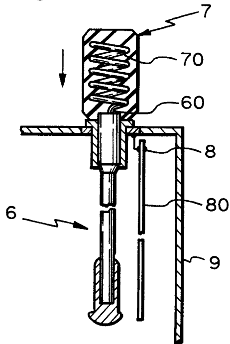
Fig. 7 PRIOR ART
