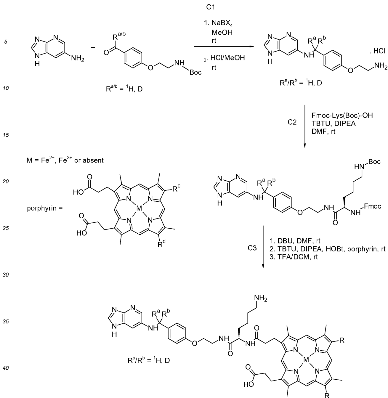
Scheme 3: Exemplary synthetic scheme for the synthesis of N-Benzylimidazo[4,5-b]pyridin-6-amine-porphyrin conjugates
