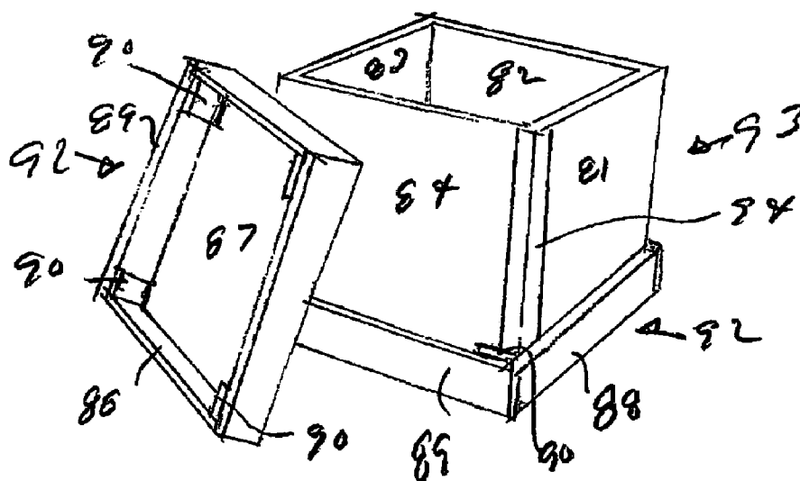
FIGURE 10 (PRIOR ART)
