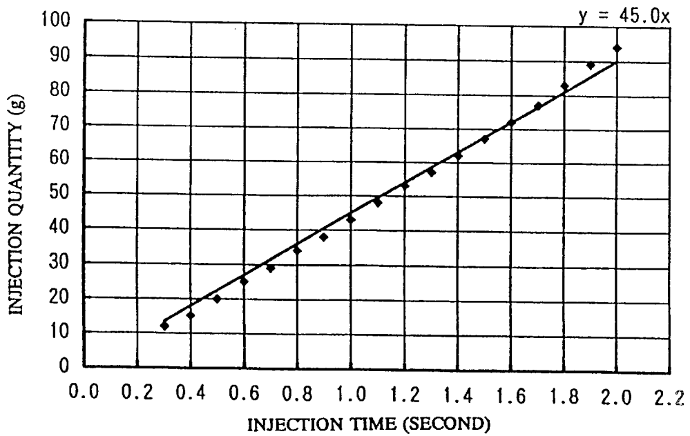
RELATIONSHIP BETWEEN INJECTION TIME AND INJECTION QUANTITY
