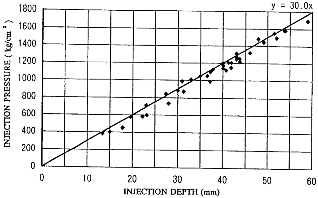
RELATIONSHIP BETWEEN INJECTION DEPTH AND INJECTION PRESSURE
