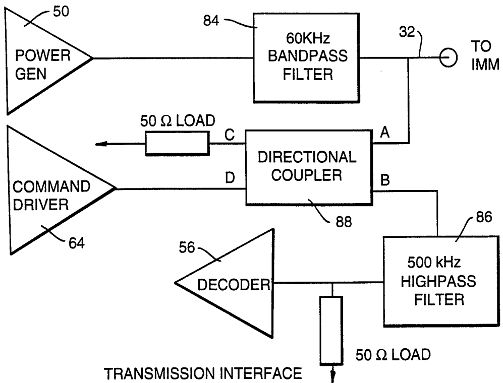
Fig.7B. SPLITTER / COMBINER, COMPLEX VERSION
