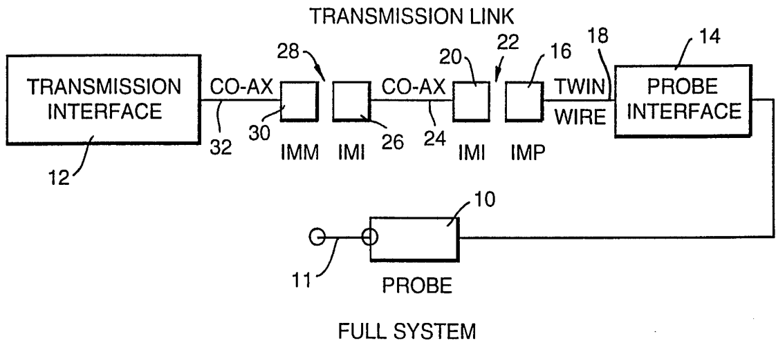
1/9 Fig. 1. COUPLING ARRANGEMENTS
