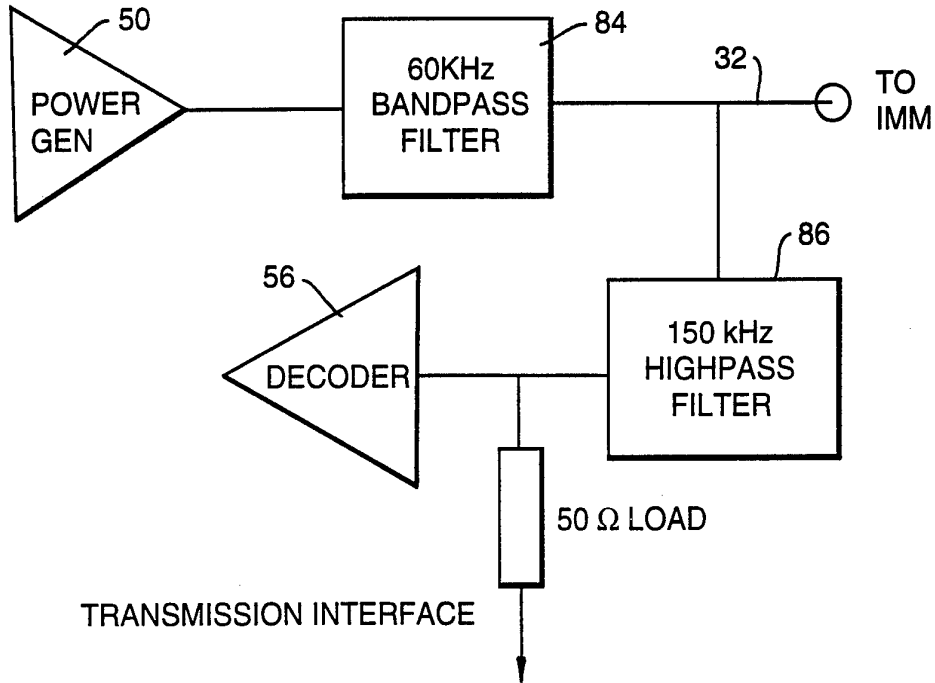
Fig.7A. SPLITTER / COMBINER, SIMPLE VERSION
