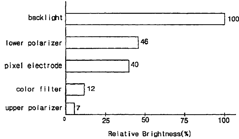
FIG. 3 (RELATED ART)
