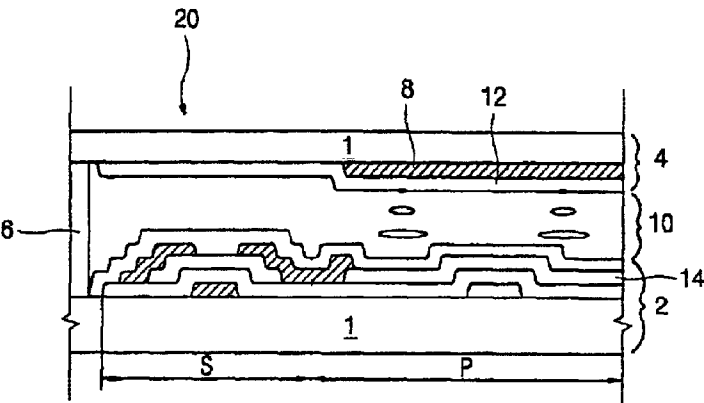
FIG. 1 (RELATED ART)
