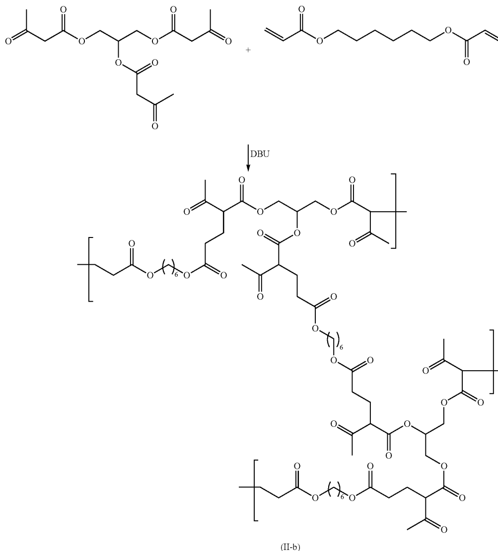
Scheme 3
