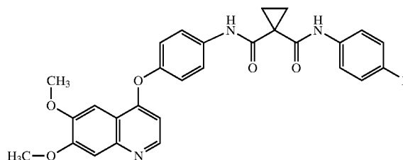
Compound 1
