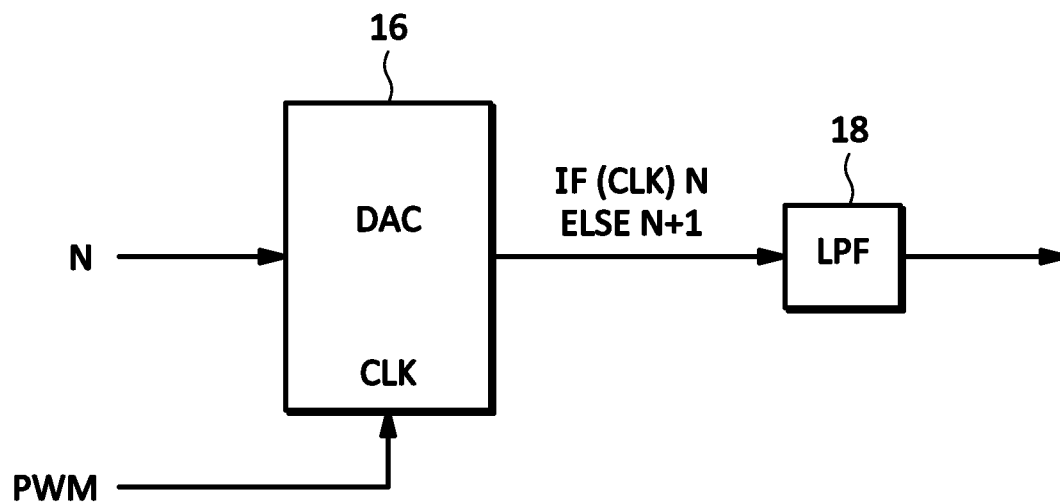
FIG. 2 (PRIOR ART)
