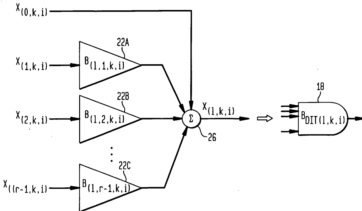
FIG. 4B SIMPLIFIED JABER'S RADIX- r DIT ENGINE
