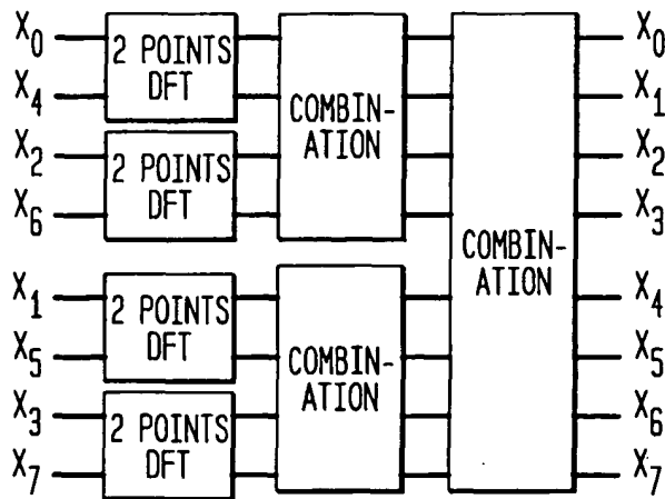
FIG. 1C (PRIOR ART)
