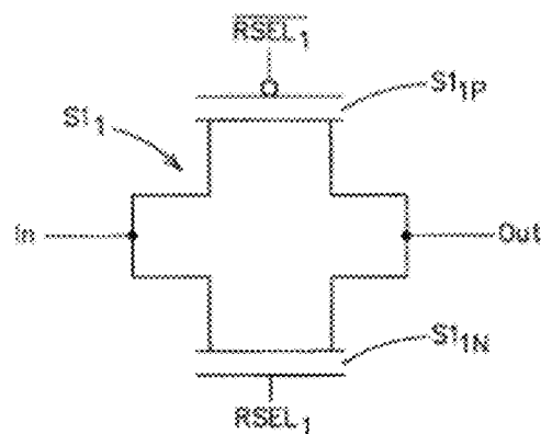
FIG. 4 (Prior Art)
