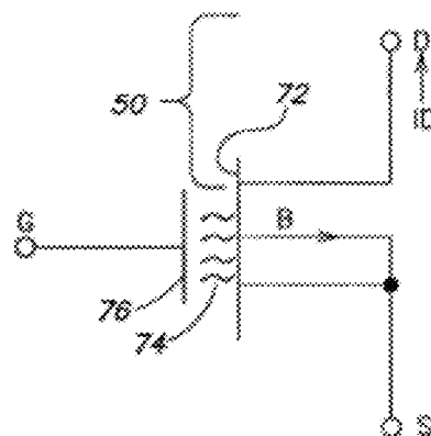
FIG. 2 (Prior Art)
