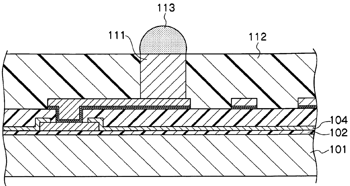
FIG. 9 PRIOR ART
