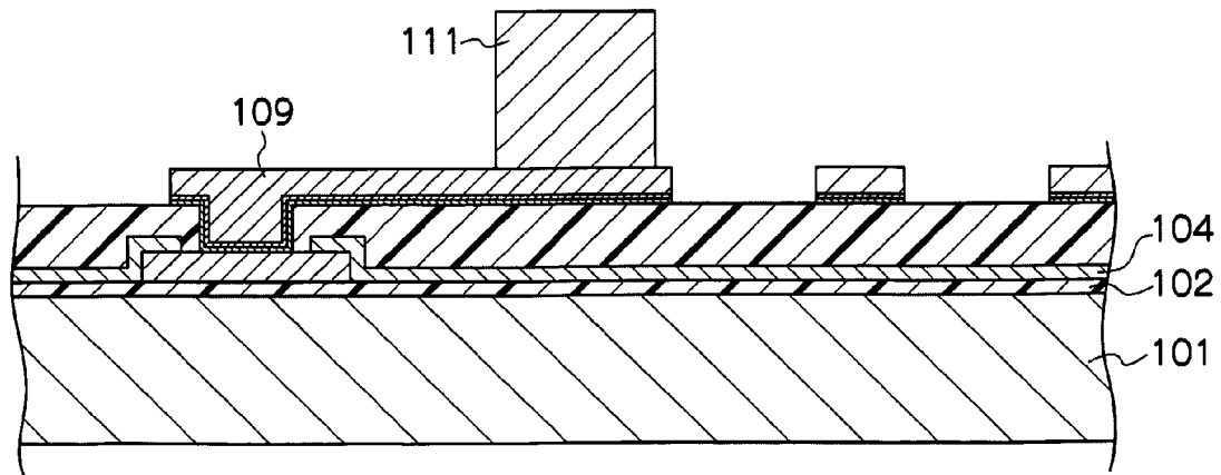
FIG. 8C PRIOR ART
