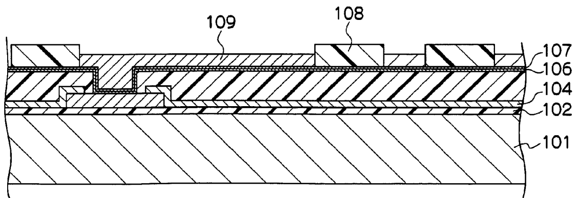
FIG. 7C PRIOR ART
