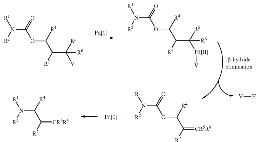
Scheme 29
