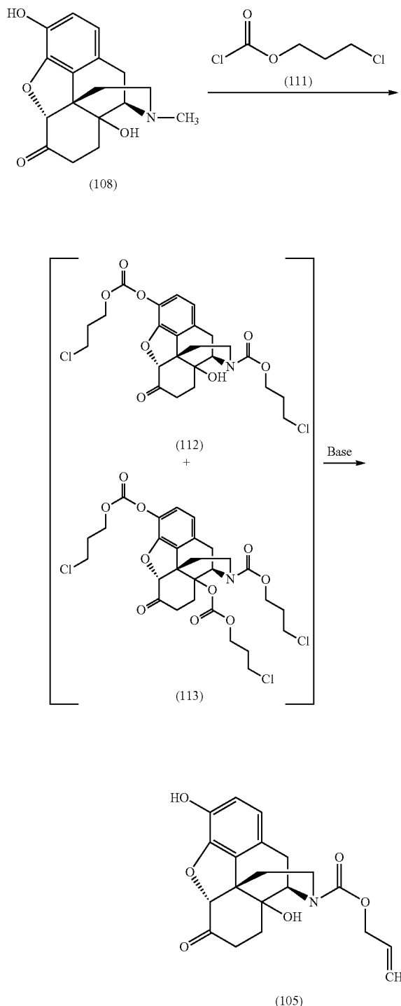
Scheme 11
