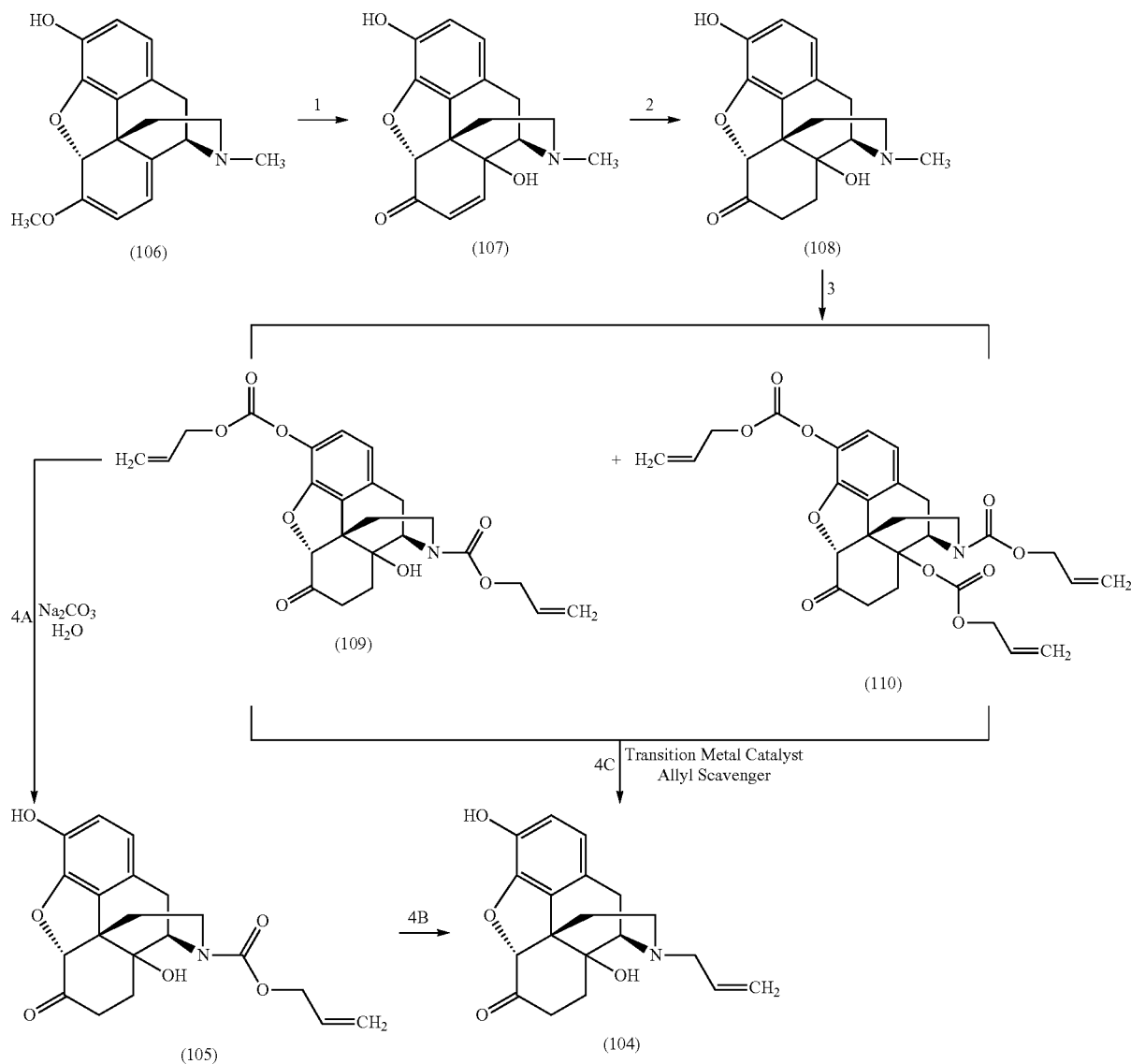
Scheme 10
