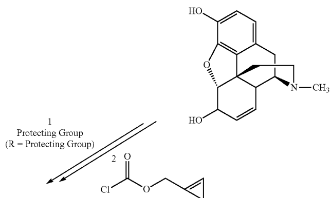
Scheme 32
