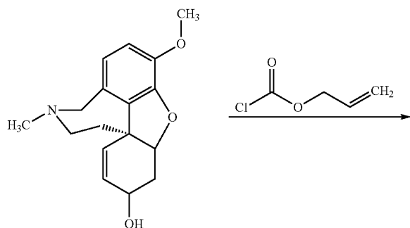
Scheme 27: Galanthamine
