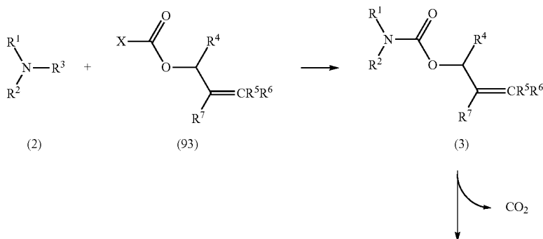
Scheme 30
