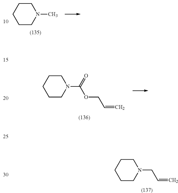
Scheme 23
