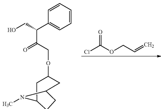
Scheme 24: Atropine
