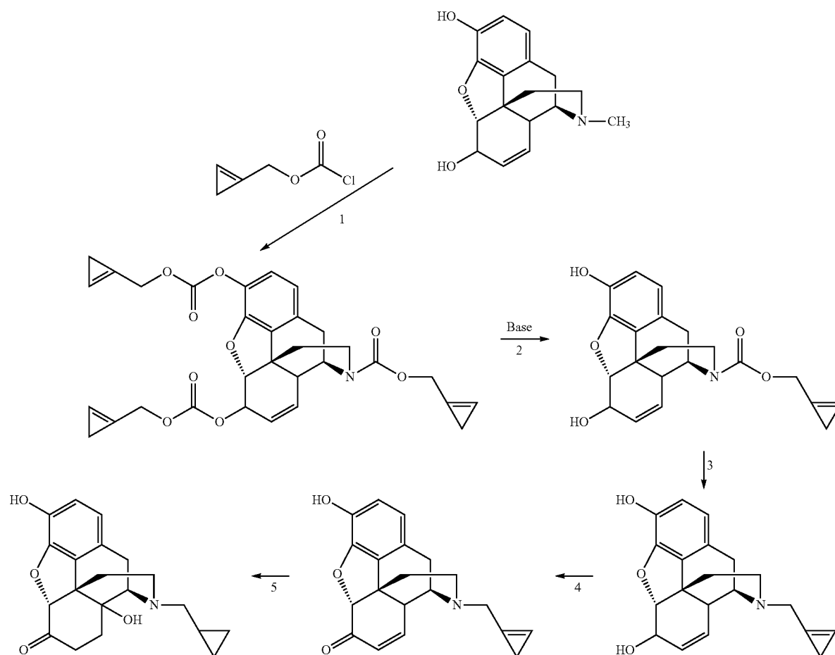
Scheme 31
