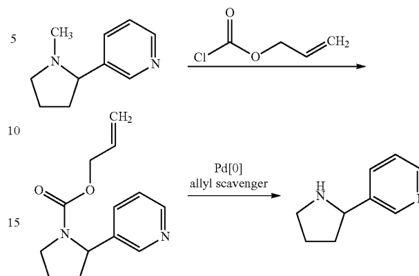
Scheme 28: Nicotine
