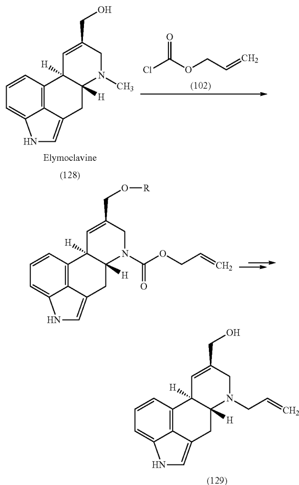
Scheme 18
