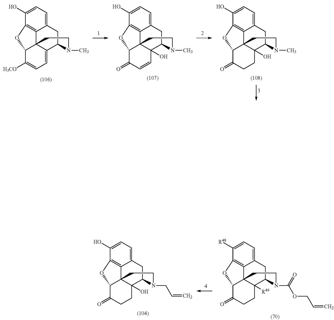
Scheme 6
