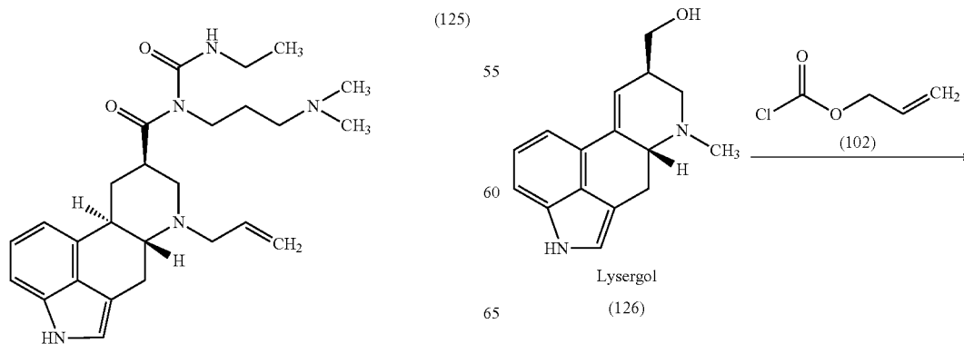
Scheme 17
