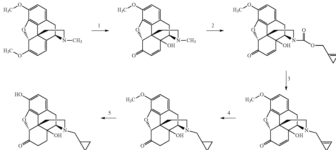
Scheme 34
