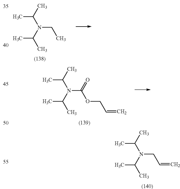
Scheme 23
