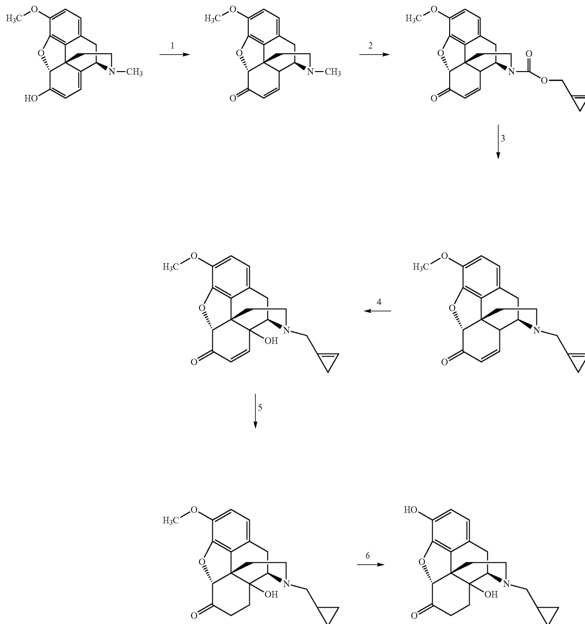
Scheme 33
