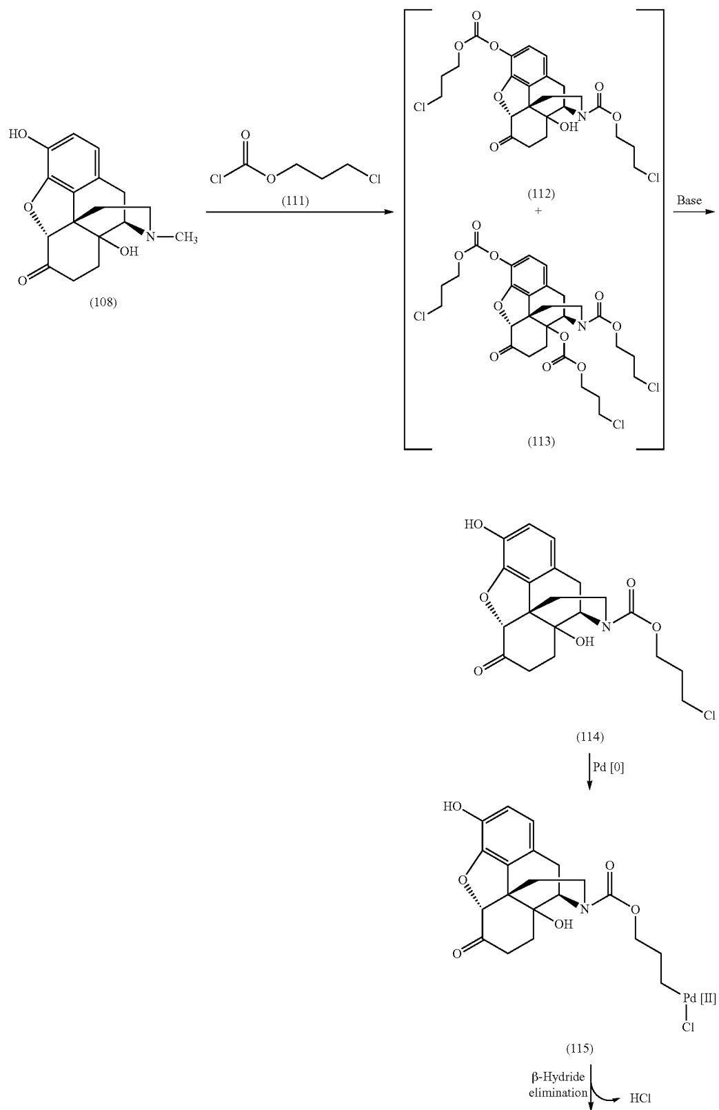
Scheme 12
