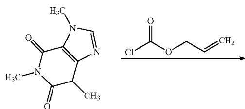
Scheme 25: Caffeine
