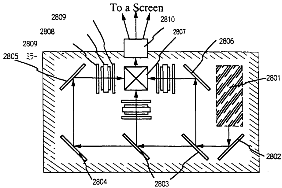
Fig. 18(C) Display Device(3 panel projector)
