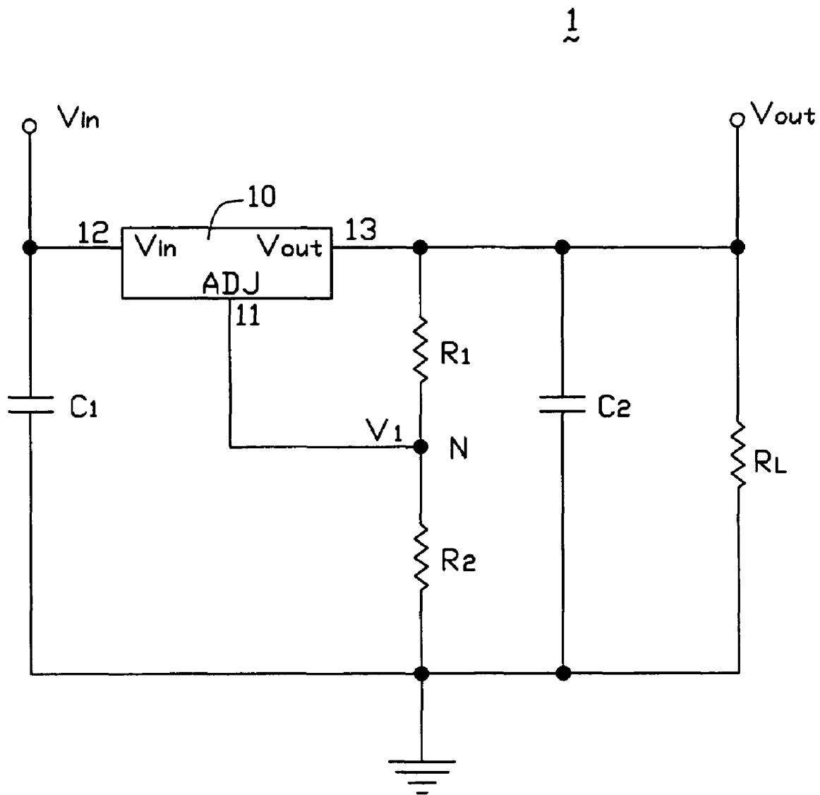
FIG. 3 (PRIOR ART)
