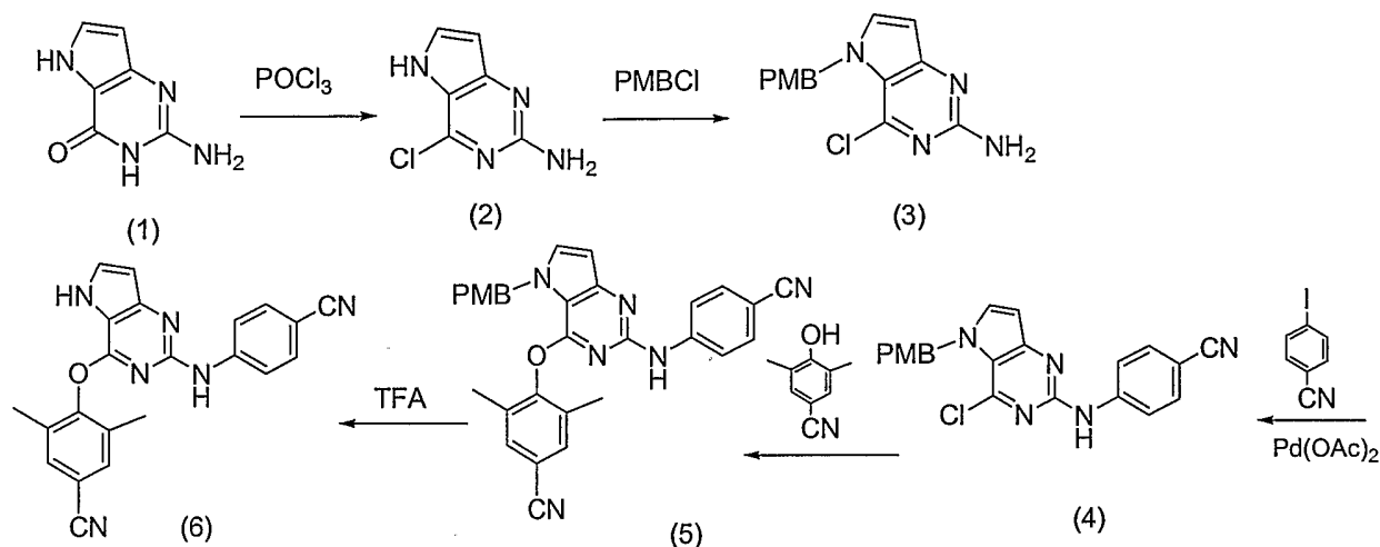
Scheme 4
