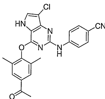
4-(4-(4-Acetyl-2,6-dimethylphenoxy)-7-chloro-5H-pyrrolo[3,2-d]pyrimidin-2-ylamino)benzonitrile
