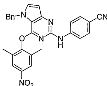
4-(5-benzyl-4-(2,6-dimethyl-4-nitrophenoxy)-5H-pyrrolo[3,2-d]pyrimidin-2-ylamino)benzonitrile
