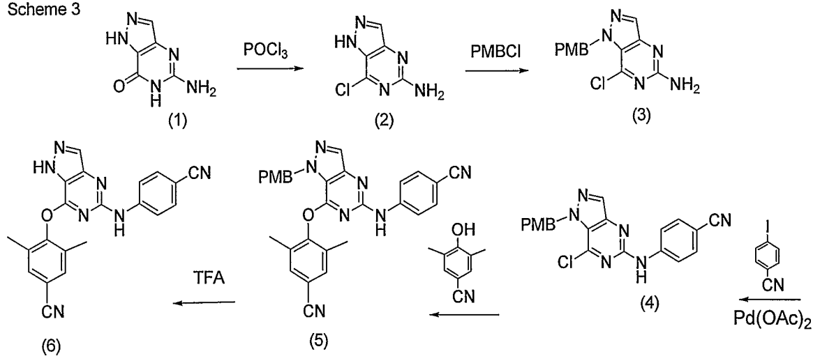
Scheme 3
