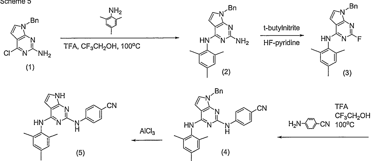
Scheme 5
