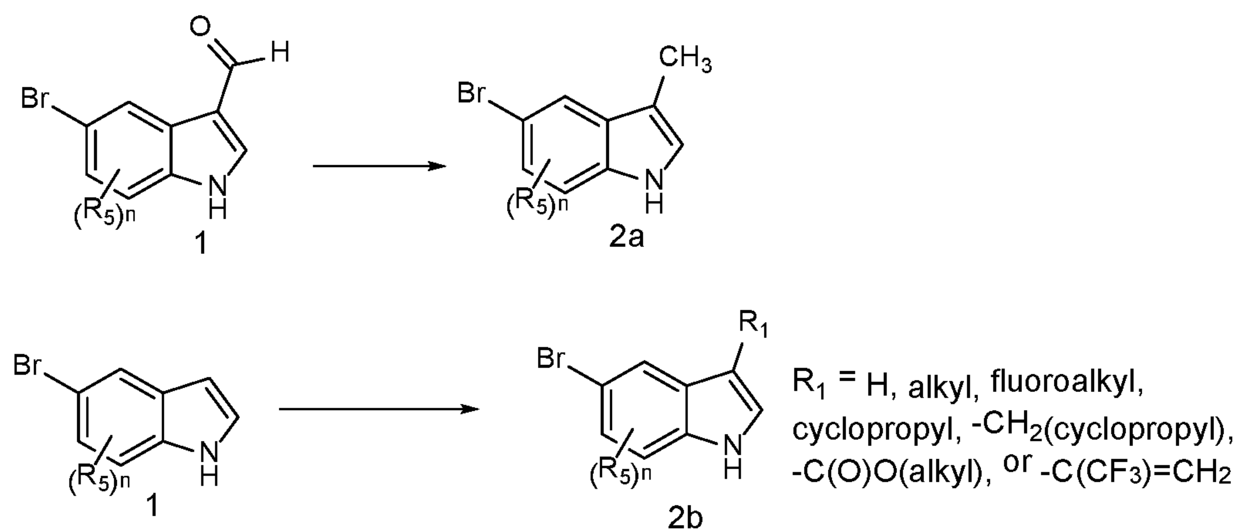
SCHEME 1
