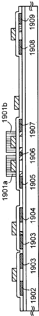
FIG. 19A STEP OF ADDING N-TYPE IMPURITY
