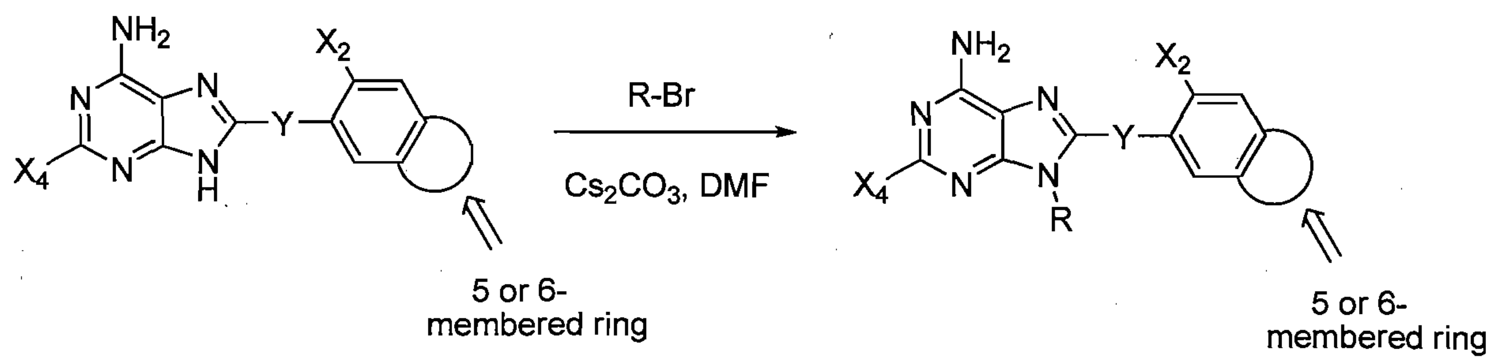
Scheme 25. Synthesis of various bromides required for alkylation of the purine skeleton.
