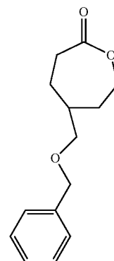
5-(Benzyloxymethyl)oxepan-2-one (BOMXO)
