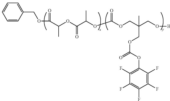
BnOH-[P(LLA-b-TMCPFP)]
