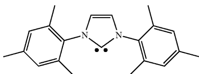
1,3-Bis(2,4,6-trimethylphenyl)imidazol-2-ylidene (Im-2)
