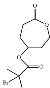
7-Oxo-oxepan-4-yl 2-bromo-2- methylpropanoate (BMP-XO)
