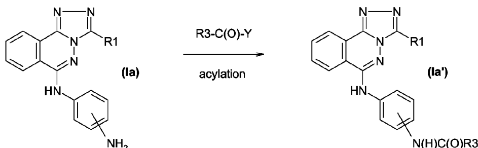
Reaction scheme 2
