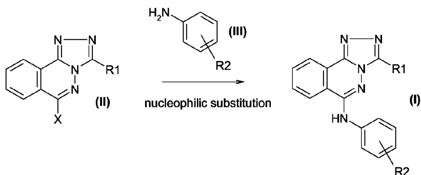
Reaction scheme 1
