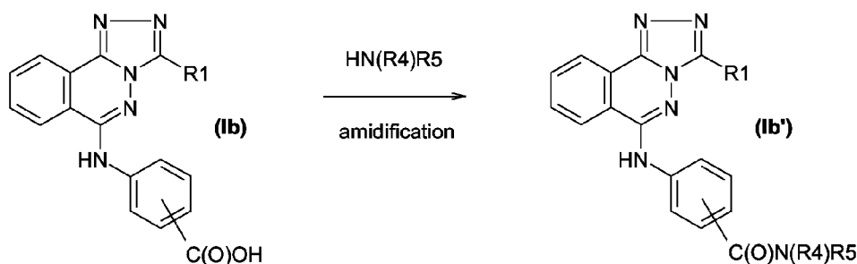
Reaction scheme 3
