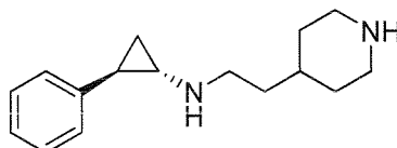
Example 69: (1R,2S)-2-phenyl-N-(2-(piperidin-4-yl)ethyl)cyclopropanamine
