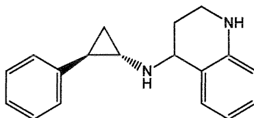
Example 62: N-((trans)-2-phenylcyclopropyl)-2-azaspiro[4.5]decan-8-amine
