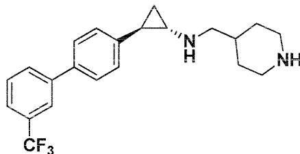
Example 81: (1R,2S)-N-(piperidin-4-ylmethyl)-2-(3'-(trifluoromethyl)-[1,1'-biphenyl]-4-yl)cyclopropanamine
