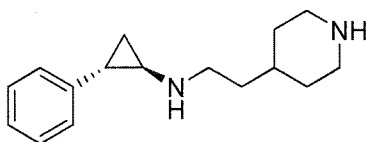
Example 70: N-((1S,2R)-2-(pyridin-3-yl)cyclopropyl)piperidin-4-amine
