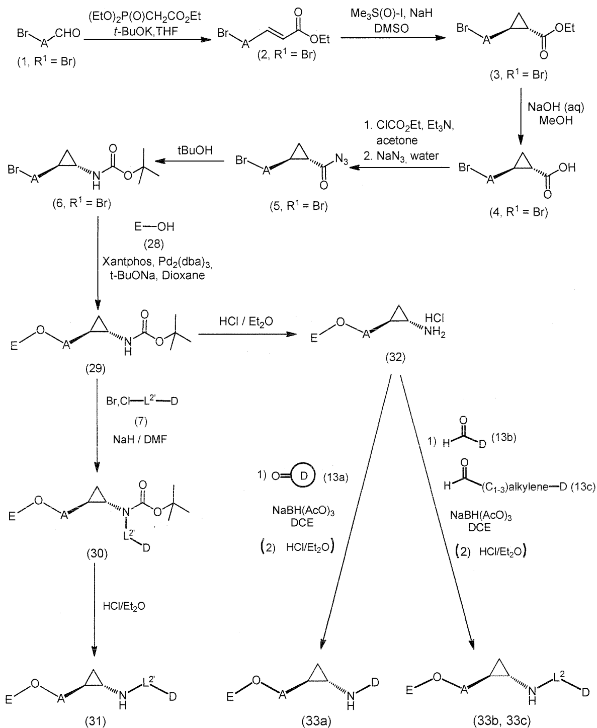
SCHEME 4: DCE (Dichloroethane), DMF (N,N-dimethylformamide), DMSO (Dimethyl sulfoxide), \text{Pd}_2(\text{dba})_3 (Tris(dibenzylideneacetone)dipalladium(0)), THF (Tetrahydrofuran), Xantphos (4,5-Bis(diphenylphosphino)-9,9-dimethylxanthene).
