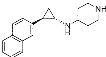
Example 96: (Trans)-2-(naphthalen-2-yl)-N-(piperidin-4-ylmethyl)cyclopropanamine
