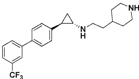
Example 89: (1R,2S)-N-(2-(piperidin-4-yl)ethyl)-2-(3'-(trifluoromethyl)-[1,1'-biphenyl]-4-yl)cyclopropanamine
