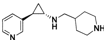
Example 77: (1R,2S)-N-(piperidin-4-ylmethyl)-2-(pyridin-3-yl)cyclopropanamine
