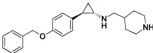
Example 83: (1R,2S)-2-(4-(benzyloxy)phenyl)-N-(piperidin-4-ylmethyl)cyclopropanamine
