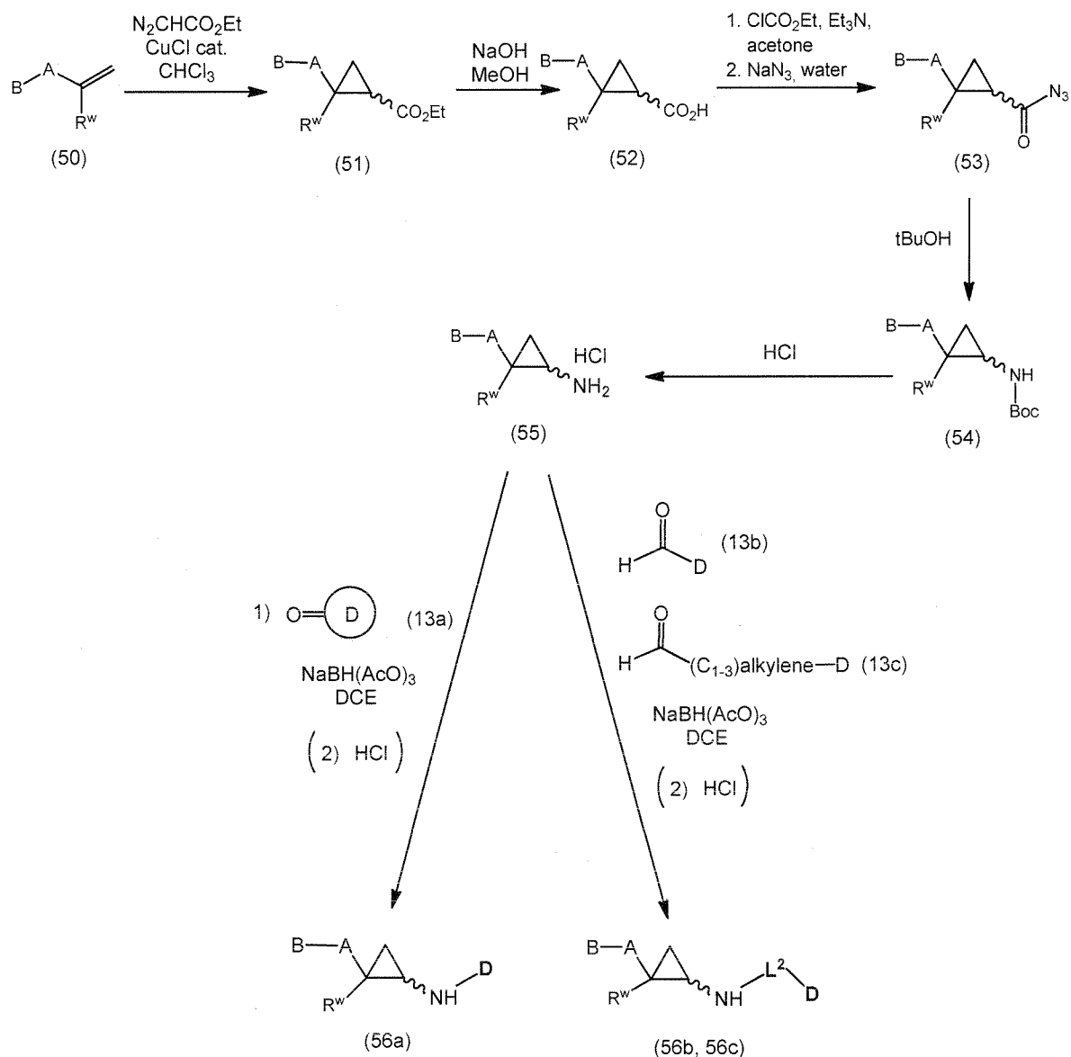
SCHEME 7: DCE (Dichloroethane)
