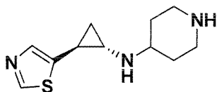
Example 73: N-((1R,2R)-2-(thiazol-5-yl)cyclopropyl)piperidin-4-amine
