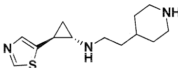
Example 87: (1R,2R)-N-(2-(piperidin-4-yl)ethyl)-2-(thiazol-5-yl)cyclopropanamine
