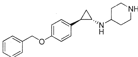
Example 65: N-((1R,2S)-2-(4-(benzyloxy)phenyl)cyclopropyl)piperidin-4-amine
