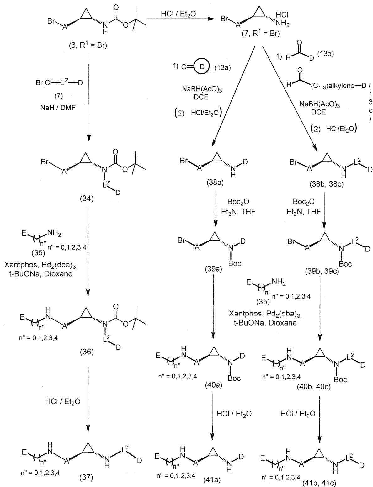
SCHEME 5: \text{Boc}_2\text{O} (Di- tert -butyl dicarbonate), DCE (Dichloroethane), DMF (N,N-dimethylformamide), DMSO (Dimethyl sulfoxide), \text{Pd}_2(\text{dba})_3 (Tris(dibenzylideneacetone)dipalladium(0)), THF (Tetrahydrofuran), Xantphos (4,5-Bis(diphenylphosphino)-9,9-dimethylxanthene).
