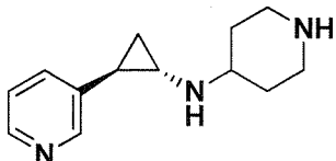
Example 71: N-((1R,2S)-2-(pyridin-3-yl)cyclopropyl)piperidin-4-amine
