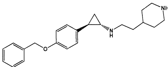
Example 53: N-((trans)-2-(3'-(trifluoromethyl)-[1,1'-biphenyl]-4-yl)cyclopropyl)piperidin-3-amine
