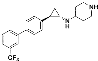
Example 75: N-((1R,2S)-2-(3'-(trifluoromethyl)-[1,1'-biphenyl]-4-yl)cyclopropyl)piperidin-4-amine
