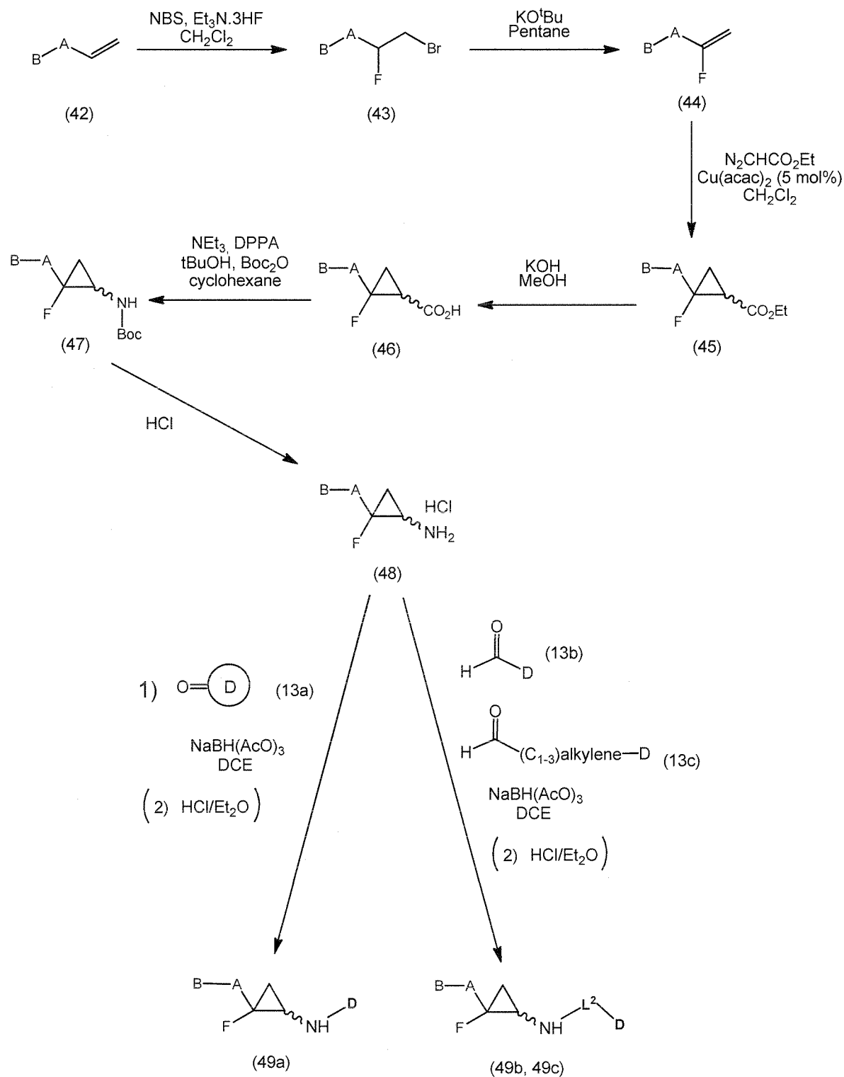
5 SCHEME 6: Boc_2O (Di- tert -butyl dicarbonate), DCE (Dichloroethane), DPPA (Diphenylphosphoryl azide), Cu(acac)_2 (Copper(II) acetylacetonate), NBS (N-Bromosuccinimide),
