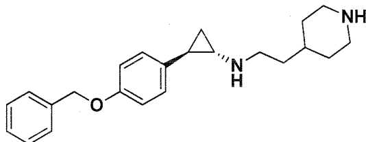
Example 91: (1R,2S)-2-(4-(benzyloxy)phenyl)-N-(2-(piperidin-4-yl)ethyl)cyclopropanamine
