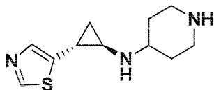
Example 74: N-((1S,2R)-2-(3'-(trifluoromethyl)-[1,1'-biphenyl]-4-yl)cyclopropyl)piperidin-4-amine
