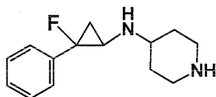
Example 93: N-((1S,2S)-2-fluoro-2-phenylcyclopropyl)piperidin-4-amine
