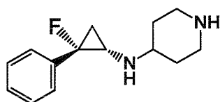
Example 94: N-((1R,2R)-2-fluoro-2-phenylcyclopropyl)piperidin-4-amine
