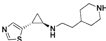
Example 88: (1S,2R)-N-(2-(piperidin-4-yl)ethyl)-2-(3'-(trifluoromethyl)-[1,1'-biphenyl]-4-yl)cyclopropanamine
