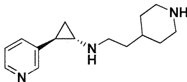
Example 85: (1R,2S)-N-(2-(piperidin-4-yl)ethyl)-2-(pyridin-3-yl)cyclopropanamine
