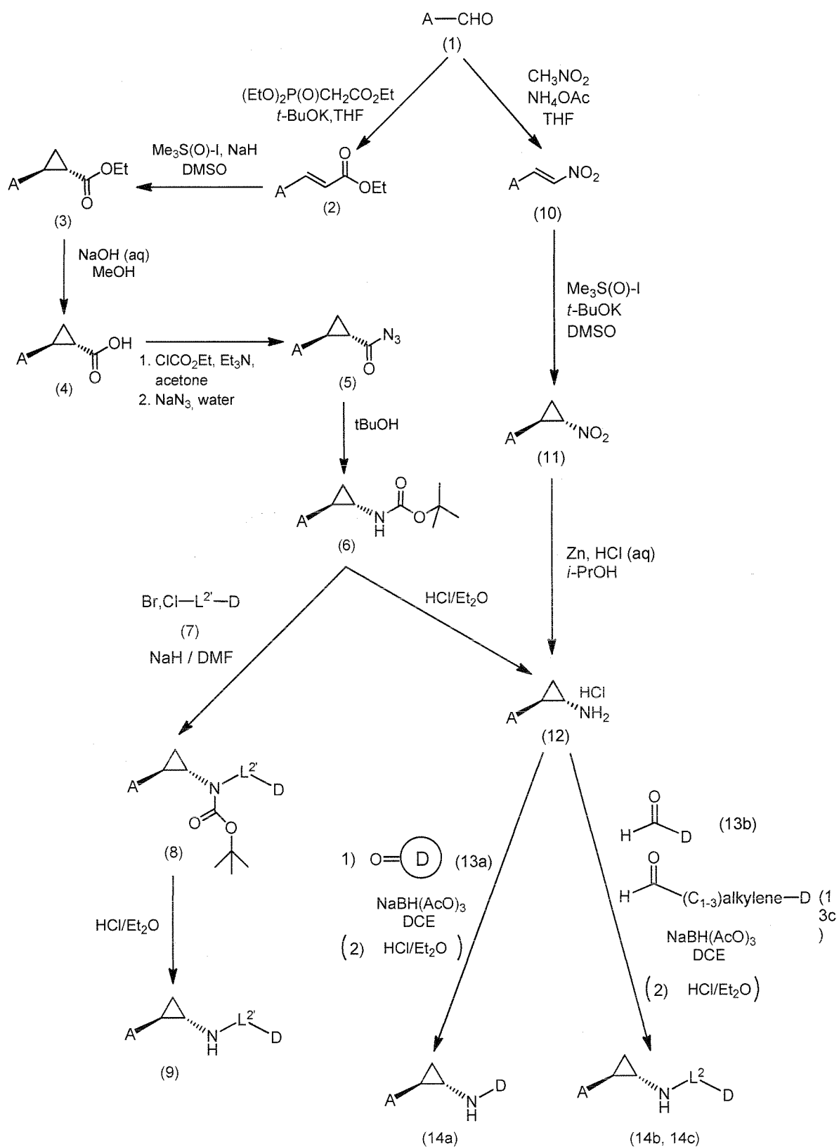
SCHEME 2: DCE (Dichloroethane), DMF (N,N-dimethylformamide), DMSO (Dimethyl sulfoxide), THF (Tetrahydrofuran). aq = aqueous.
