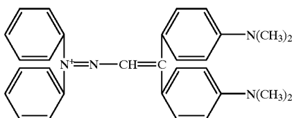
1,1-bux-[4-(N,N-dimethylamino)phenyl-3,4-bis-(phenyl)]-3,4-diazo butene carbonium (Code PP 2030)
