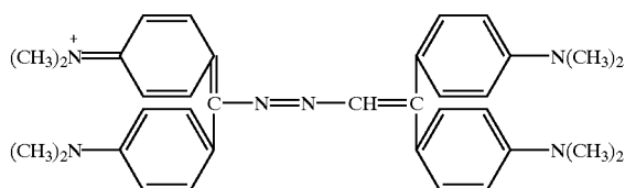
1,1,5,5-tetrakis-[4-(N,N-dimethylamino)phenyl]-2,3-diazo pentene carbonium (Code PP2031)
