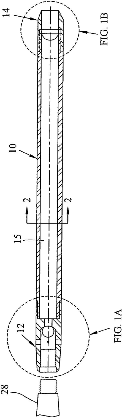
FIG. 1 PRIOR ART
