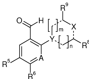
formula XIII,
