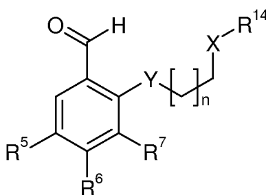
formula VIII
