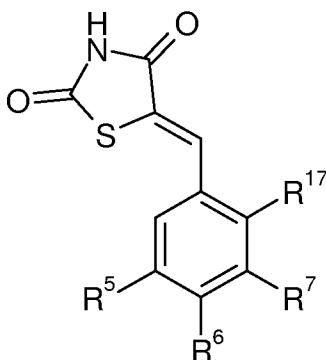
formula IX,
