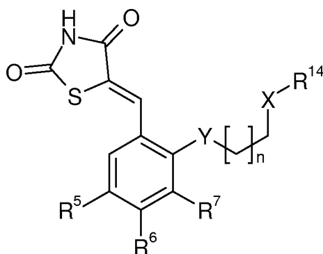
formula IC,
