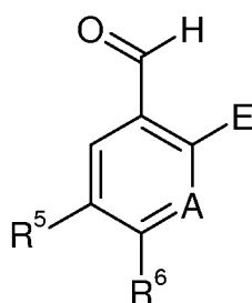
formula XI,
