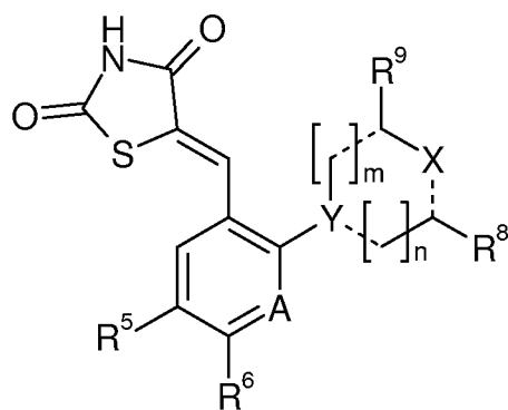
formula IA,
