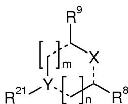
formula XII,
