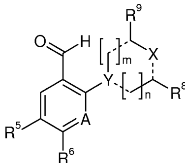
formula XIII,
