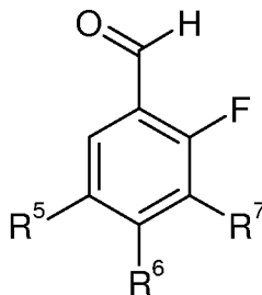
formula V,
