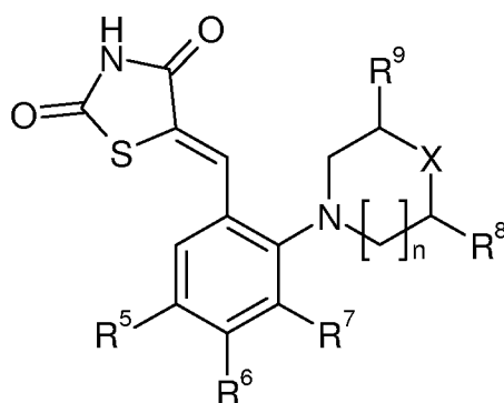
formula IB,
