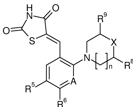
formula ID,
