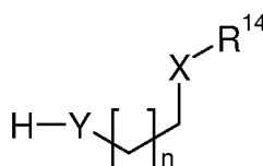
formula VII,
