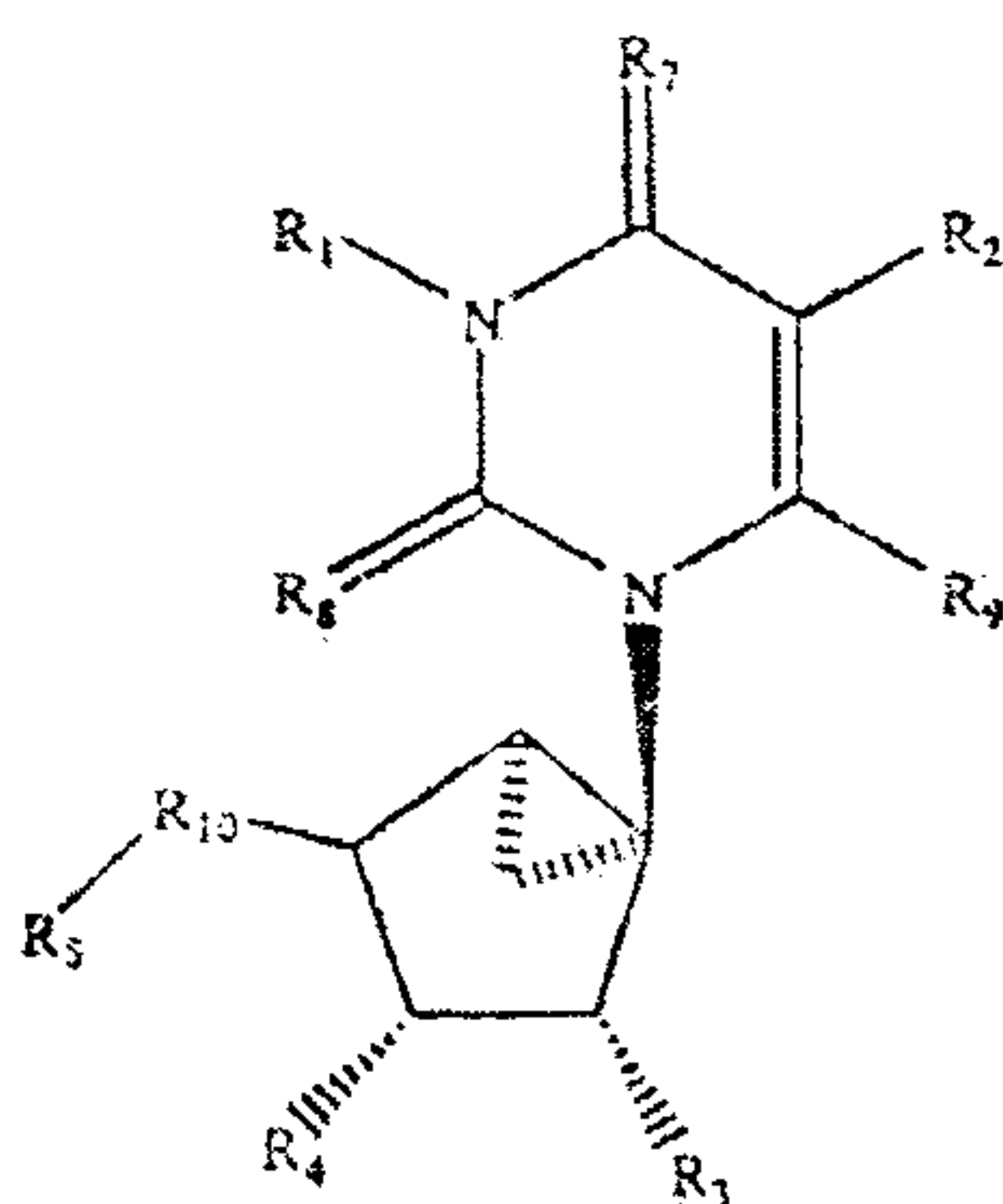
Formula IV
