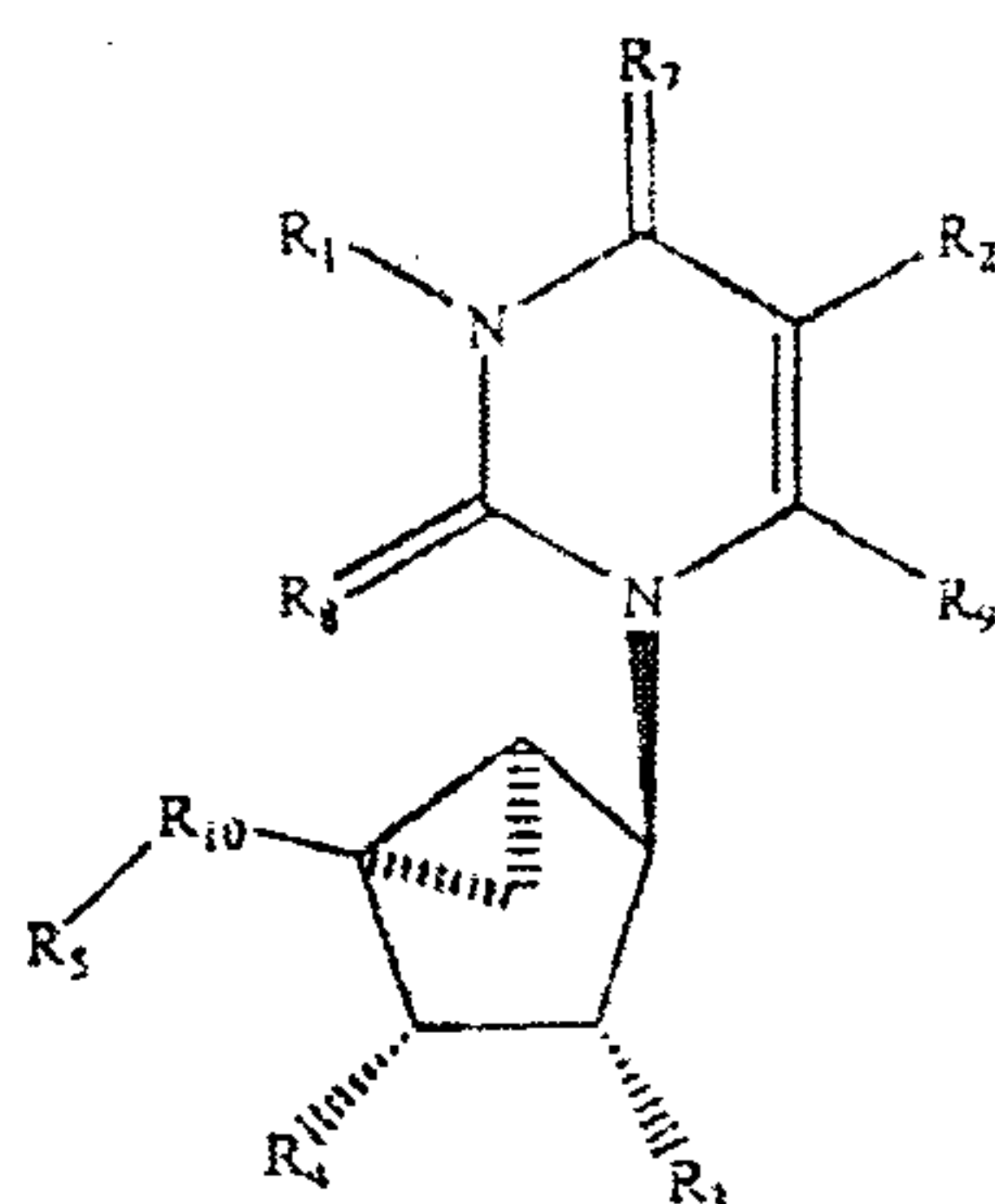
Formula III
