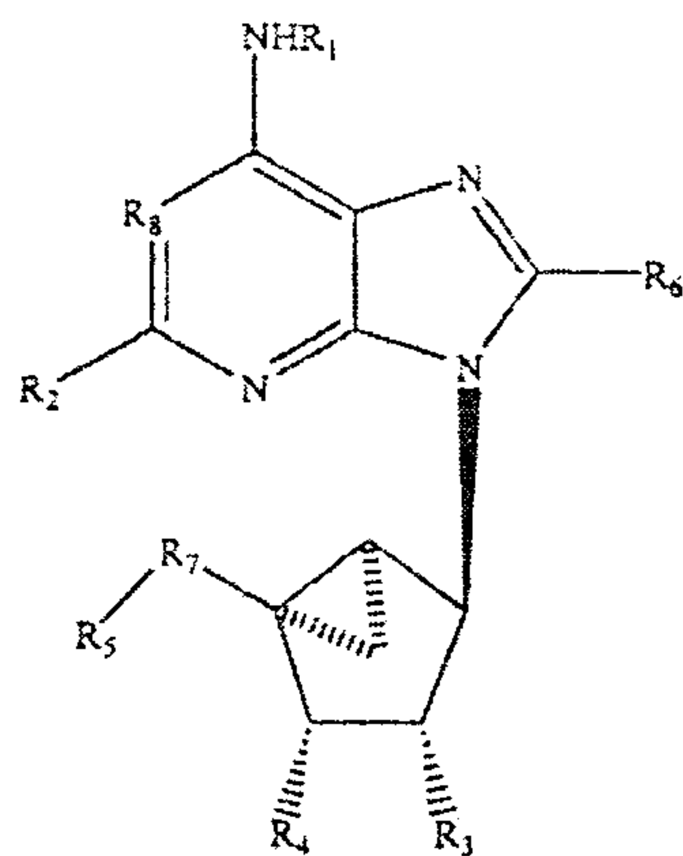
Formula 1
