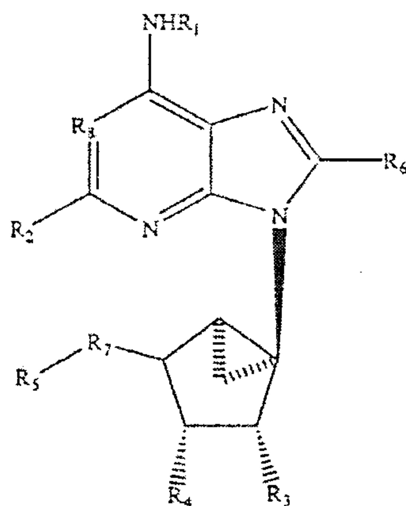
Formula II
