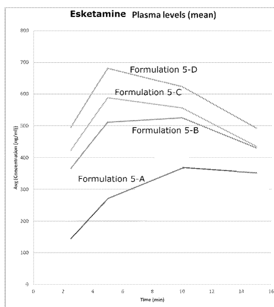
Figure 1: Esketamine Plasma Levels, rat pK Study Dosing Formulations 5-A through 5-D @ 10 µL/rat
