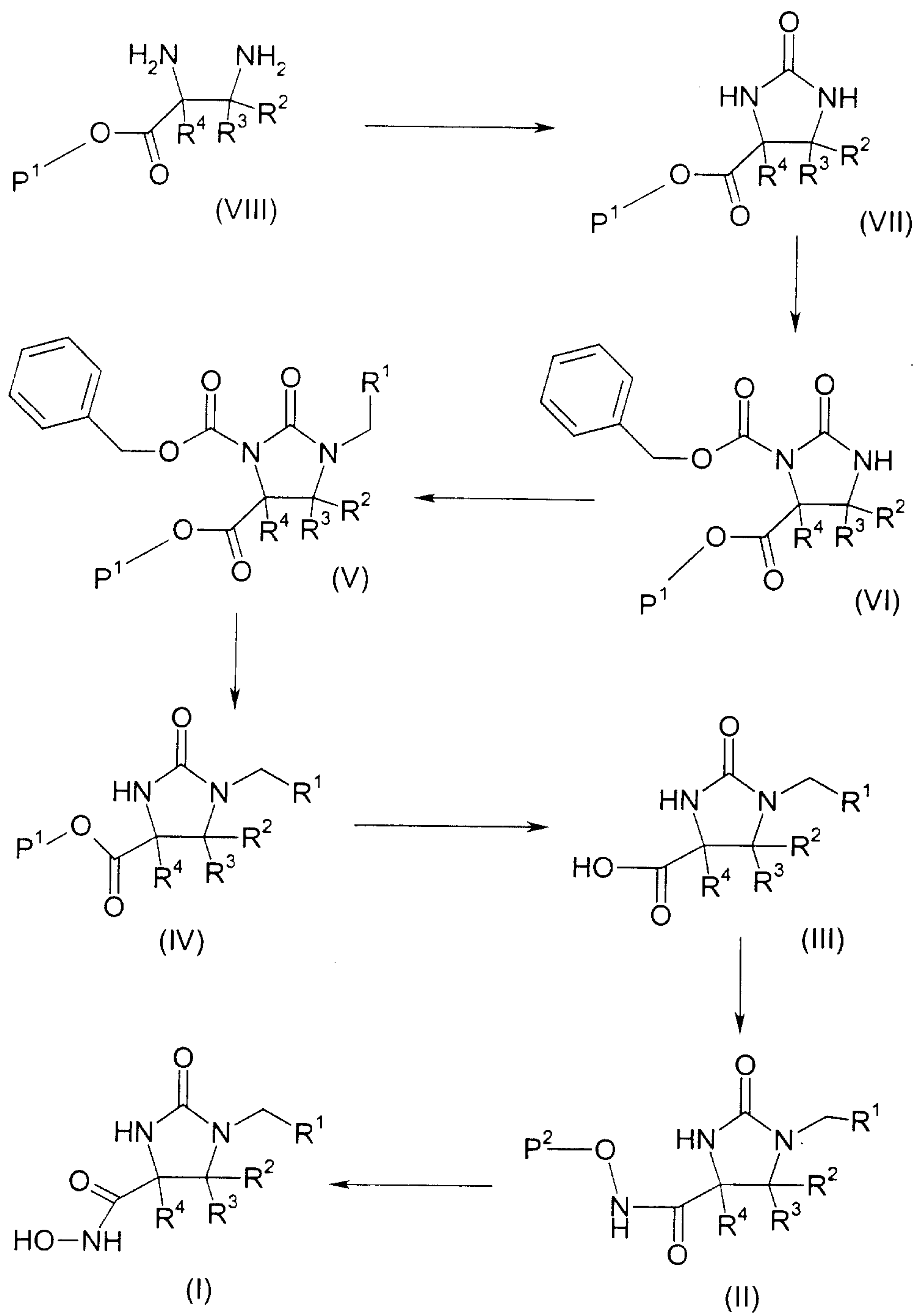
Scheme 1
