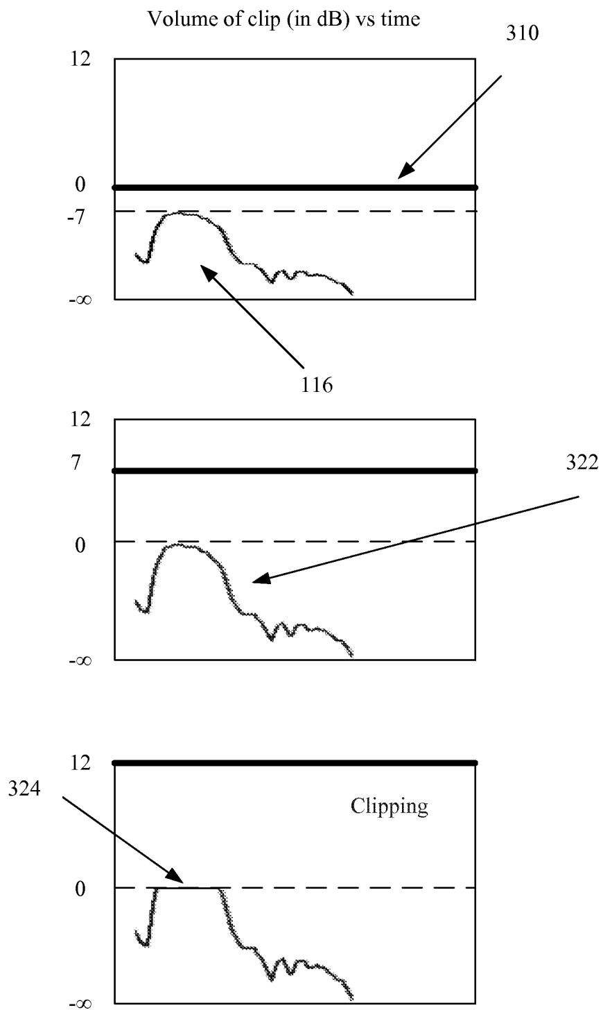
FIGURE 3 (Prior Art)
